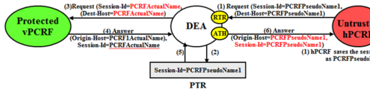
Figure 10-18 Untrusted-hPCRF to Protected-vPCRF Diameter Transaction
