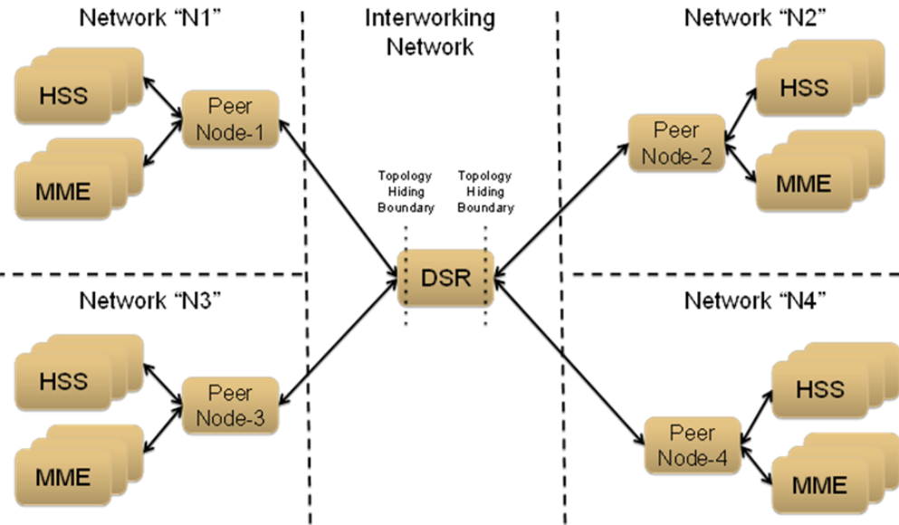
Figure 10-4 TH Network Deployment in an Interworking Network
