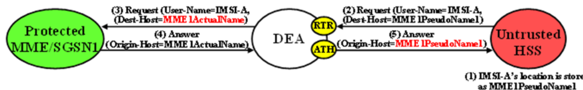
Figure 10-16 MME/SGSN TH Untrusted-HSS to Protected MME/SGSN Transaction
