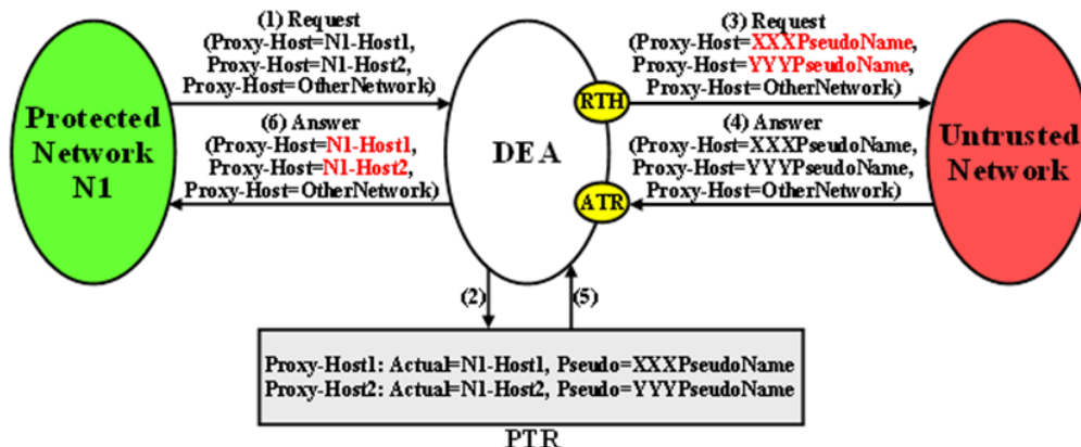
Figure 10-10 Proxy-Host Hiding
