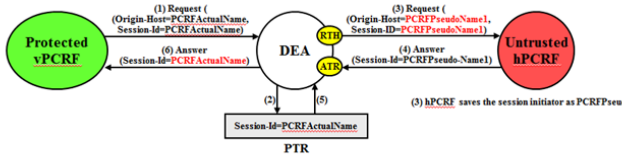
Figure 10-17 Protected-vPCRF to Untrusted-hPCRF Transaction
