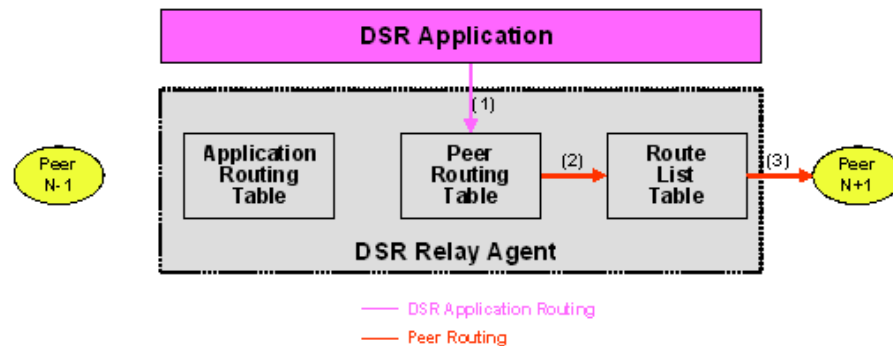
Figure 3-20 PCA Generated Request Routing
