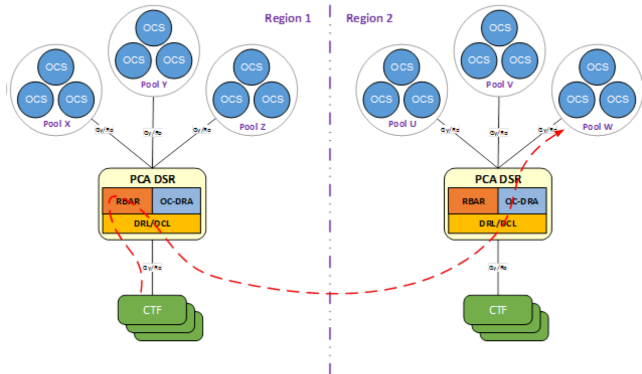
Figure 5-3 Regionalized OCS Server Pool Selection
