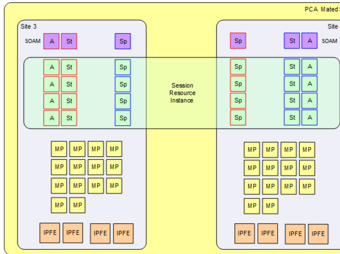
Figure 3-7 illustrates example relationships between PCA DSR Sites and Policy Clients and PCRFs:
