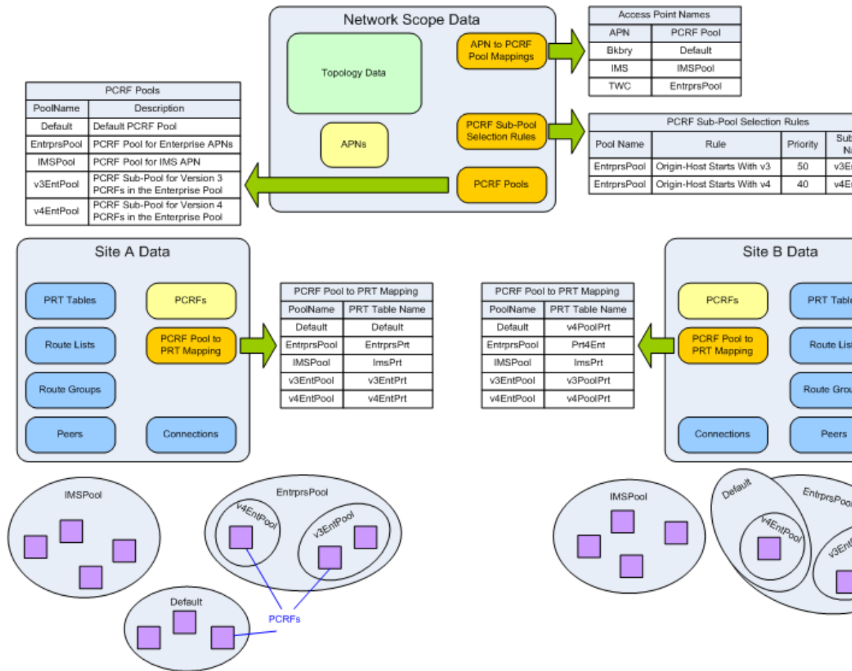
Figure 6-2 PCRf Pooling Data
