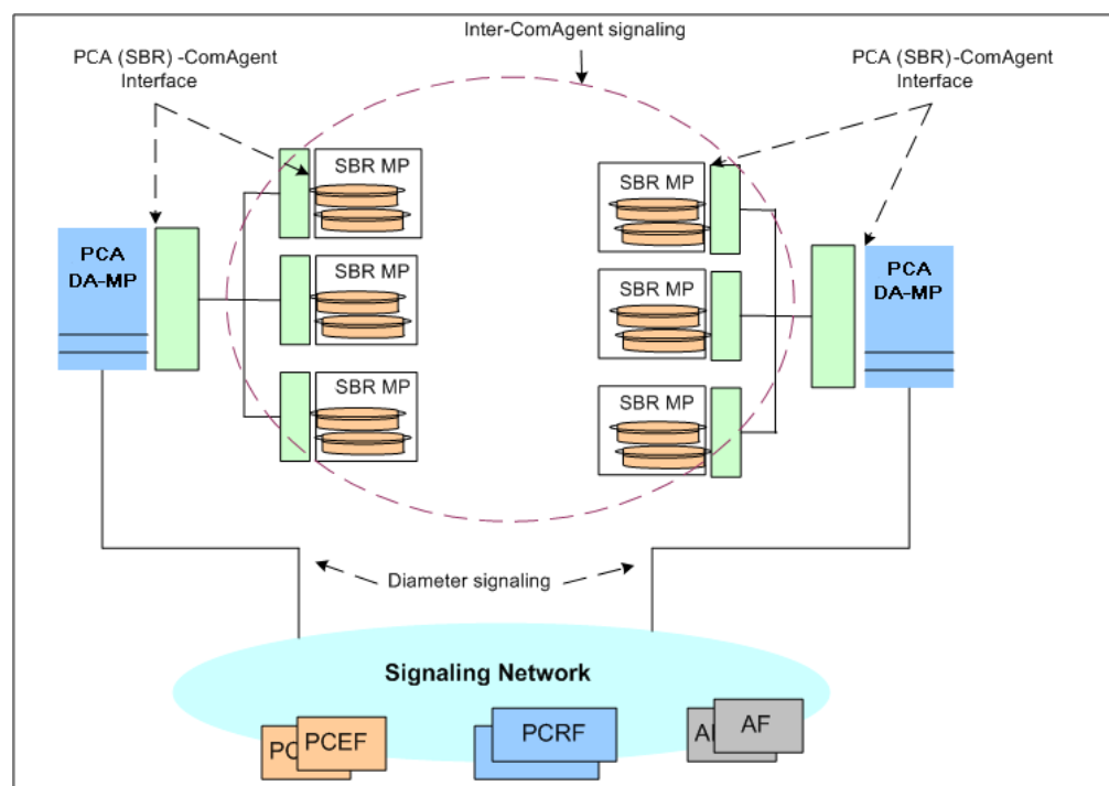
Figure 3-16 Communication between ComAgents, Policy DRA, and SBR
