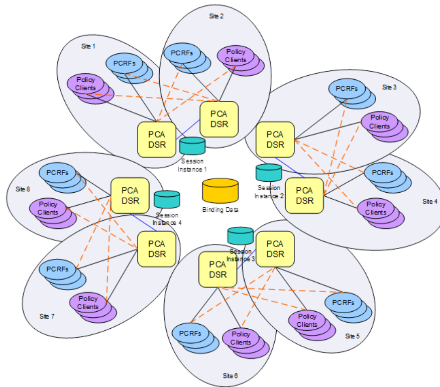
Figure 3-7 Policy Client, PCRF, and Site Relationships
