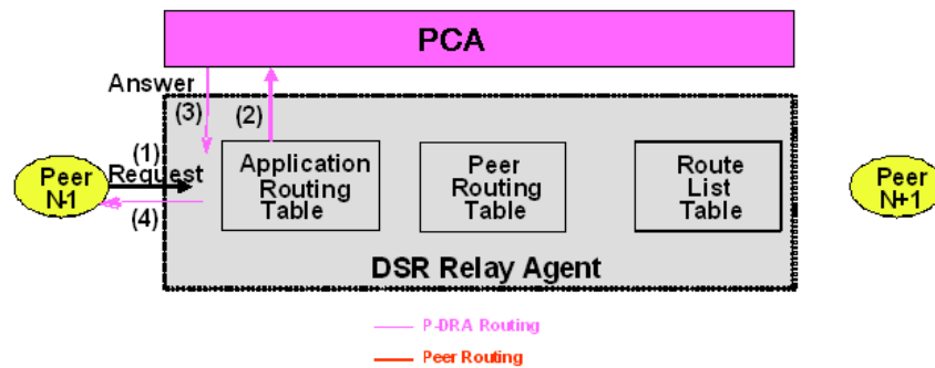
Figure 3-19 PCA Generated Answer Routing
