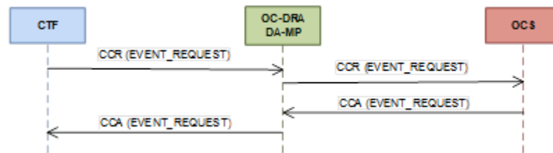
Figure 3-1 Example of Gy/Ro Event-Based Charging
