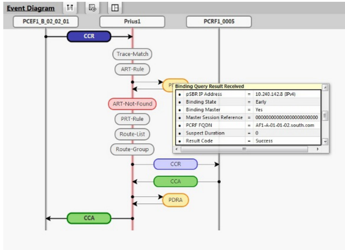
Figure 3-23 Event Diagram – Hover (Mouse-over) Example
