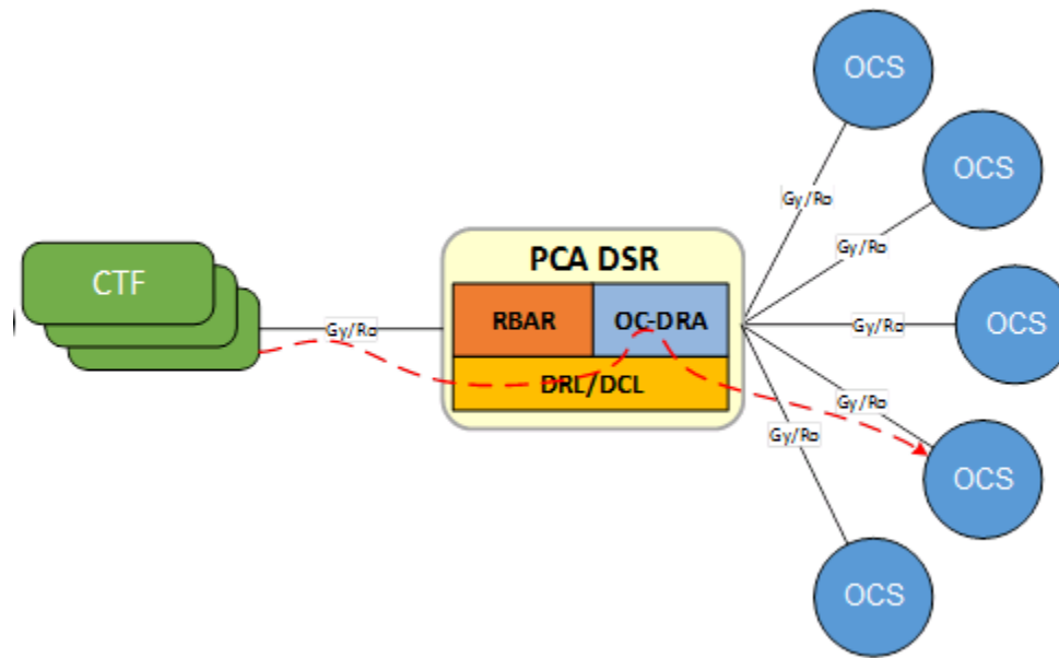
Figure 5-1 Local OCS Server Selection
