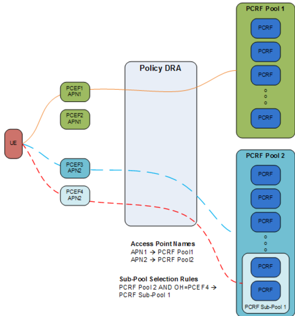
Figure 4-5 PCRF Pools and Sub-Pools Routing Scenarios
