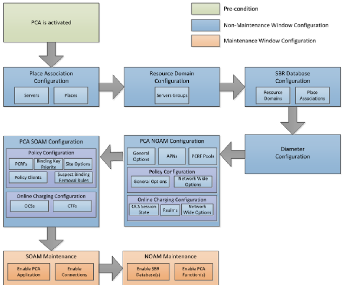
Figure 6-1 PCA Configuration Flow
