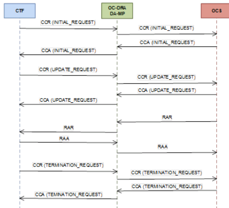
Figure 3-2 Example of Gy/Ro Session-Based Charging
