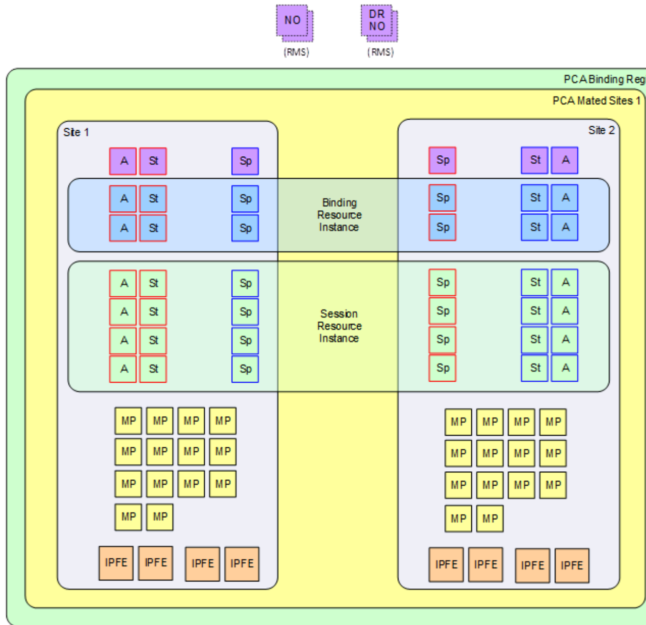
Figure 3-5 Example PCA Mated Pair - Hosting Binding SBRs
