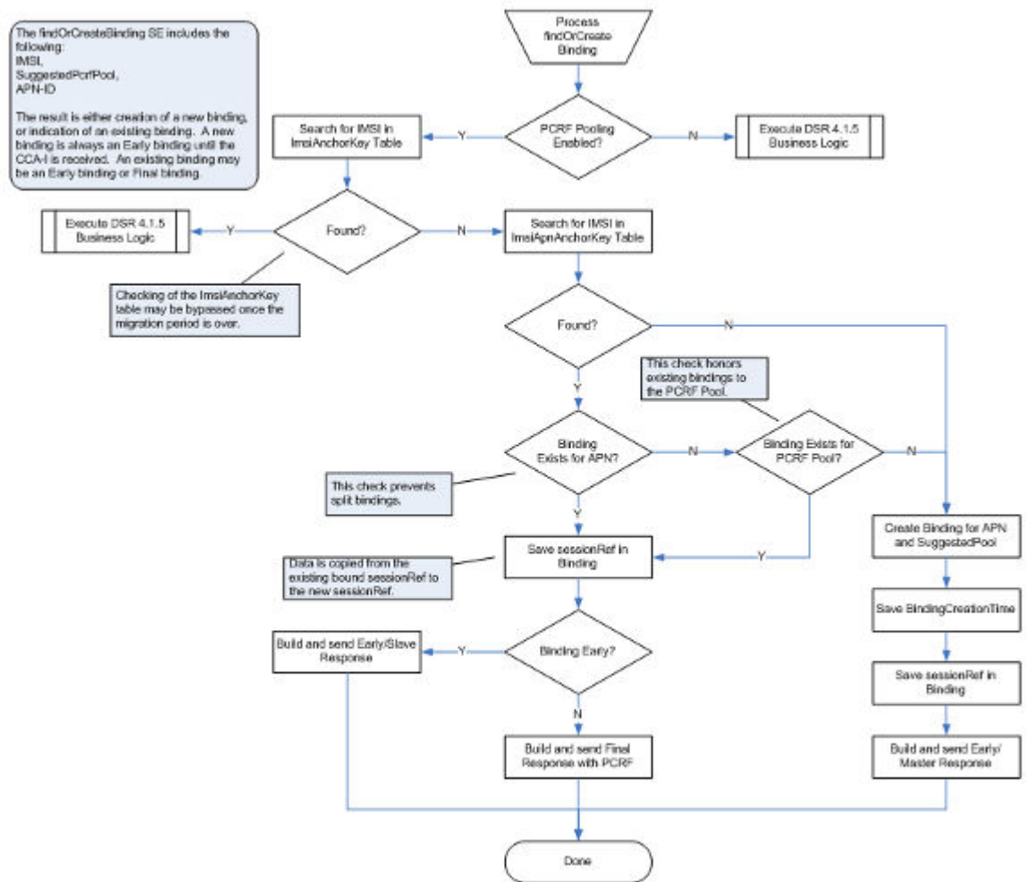
Figure 4-7 Find or Create a Binding
