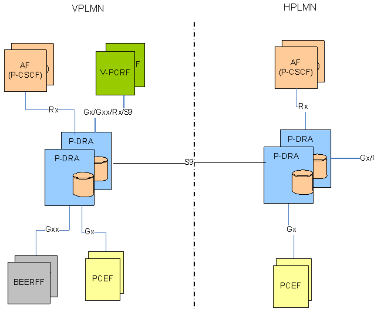
Figure 3-4 Policy DRA in Roaming Scenarios
