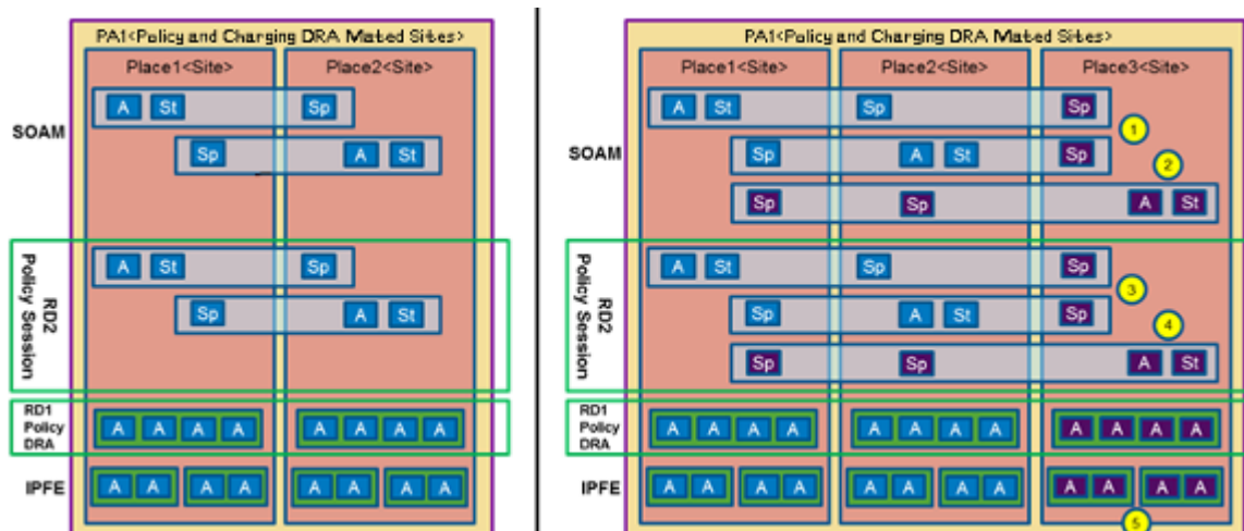
Figure 3-11 Comparing 2-Site and 3-Site Redundancy
