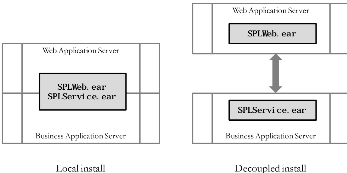
Figure 26 – Installation Modes
