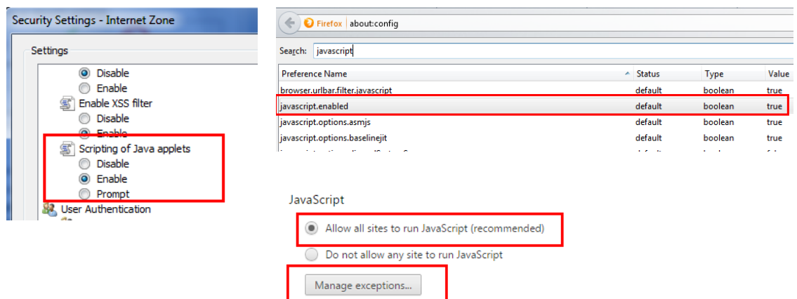
Figure 21 – Javascript Settings
