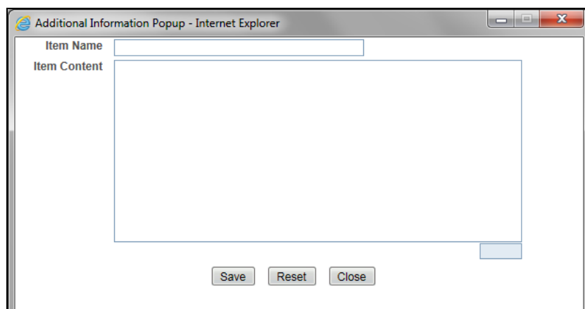
Figure 23. Additional Information
