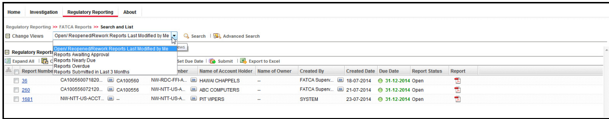
Figure 8. Views Search
