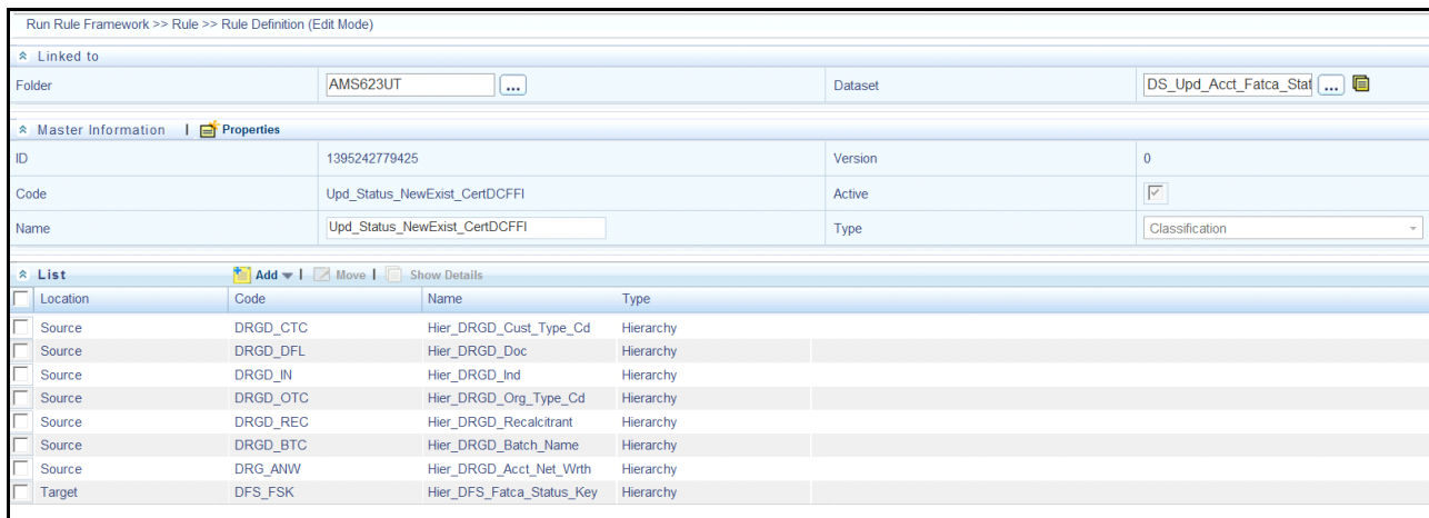
Figure 47. Rule Definition (Edit Mode)
