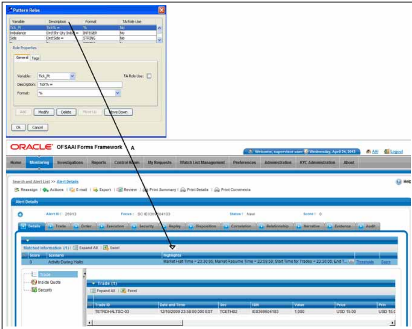
Figure 72. UI Mapping Sample- Pattern Role Editor to Alert List
