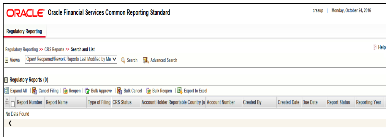
Figure 8. Views Search
