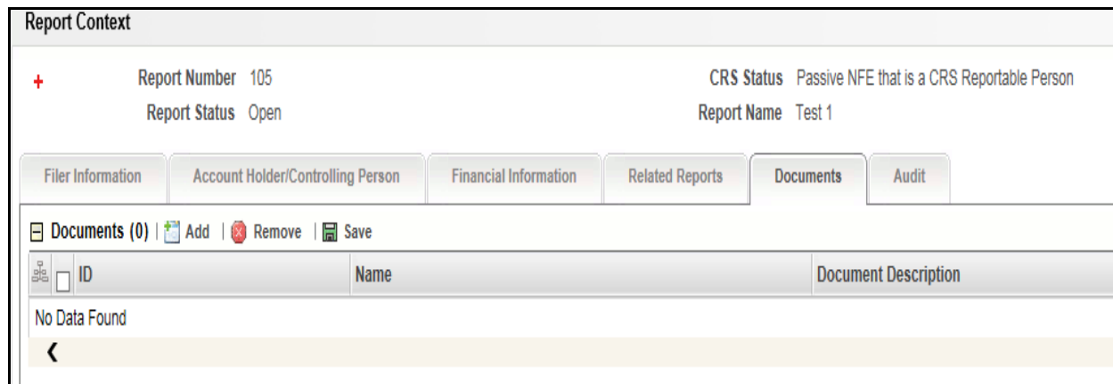
Figure 19. Documents Tab
