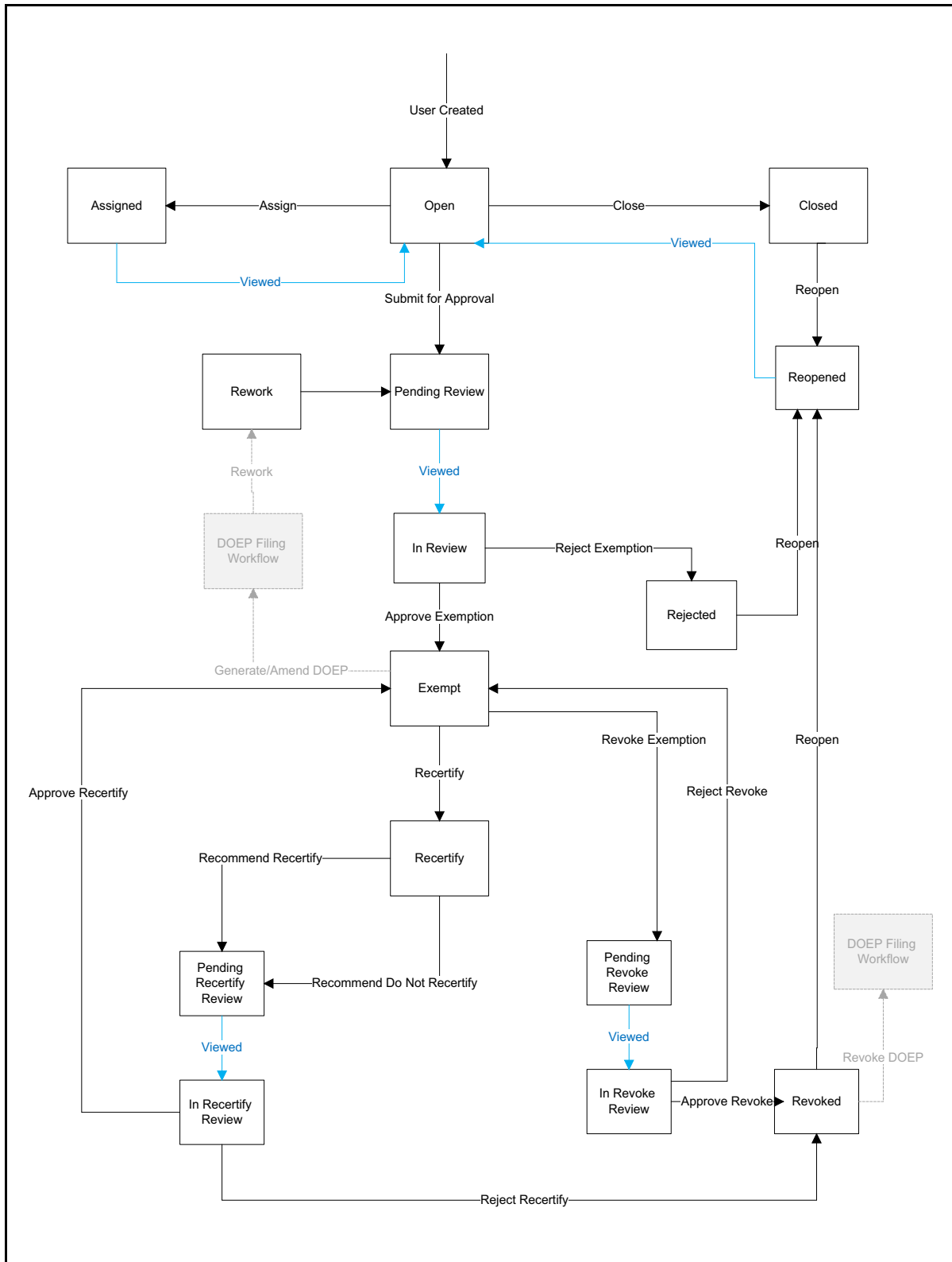
Figure 45. Exemption Workflow
