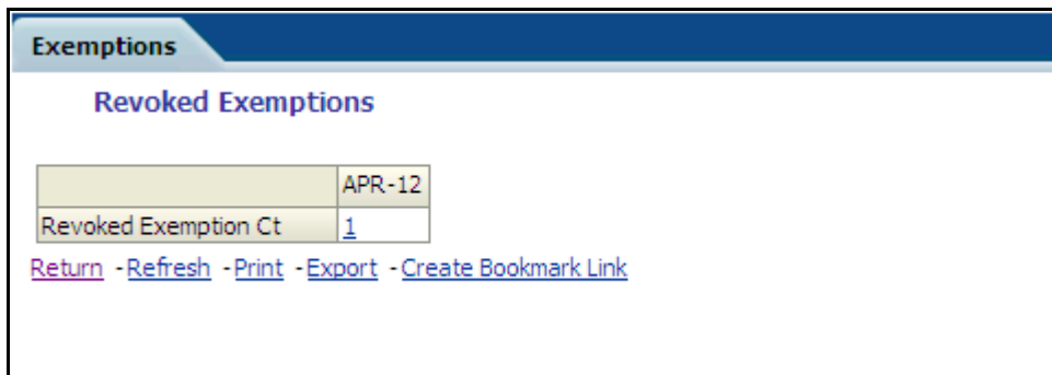
Figure 90. Revoke Exemption
