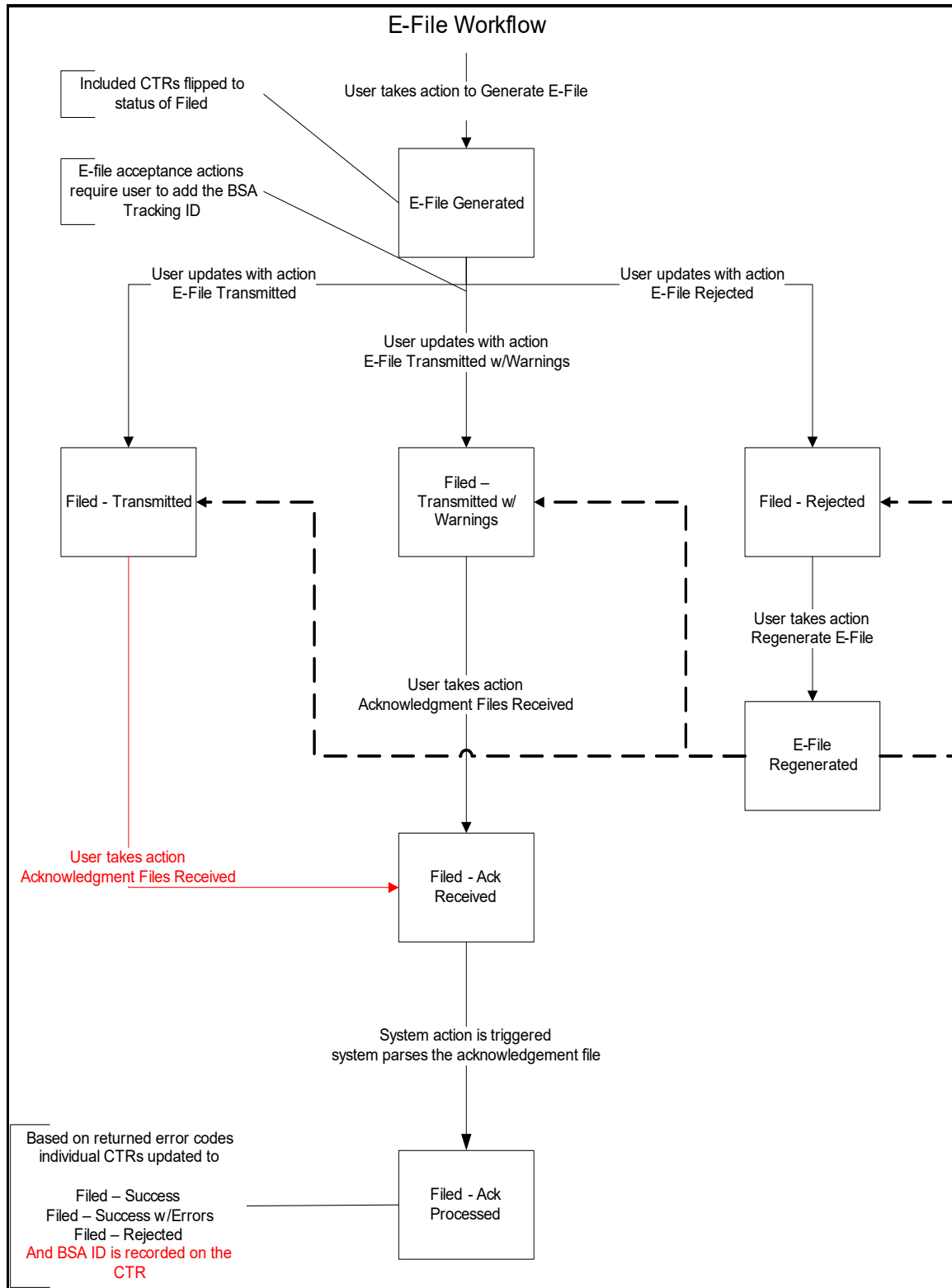
Figure 31. E-File Workflow
