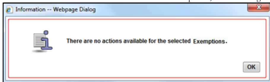
Figure 51. Actions Window
