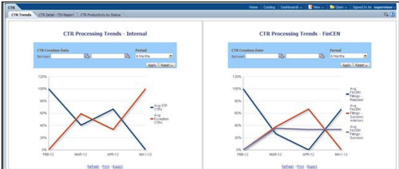
Figure 84. CTR Trends
