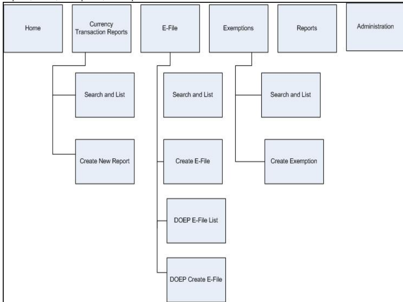
Figure 5. CTRs Menus
