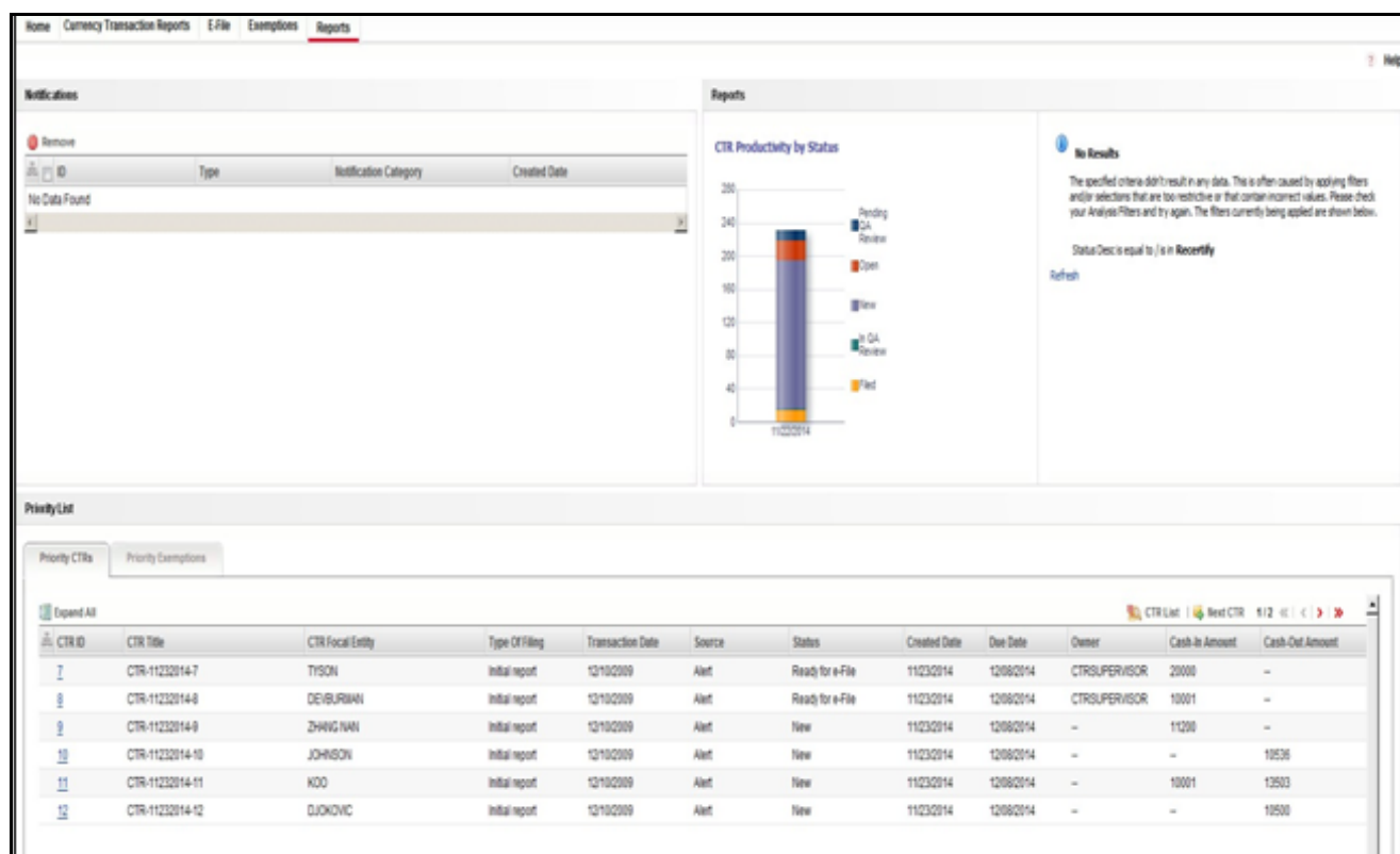
Figure 80. Accessing Reports
