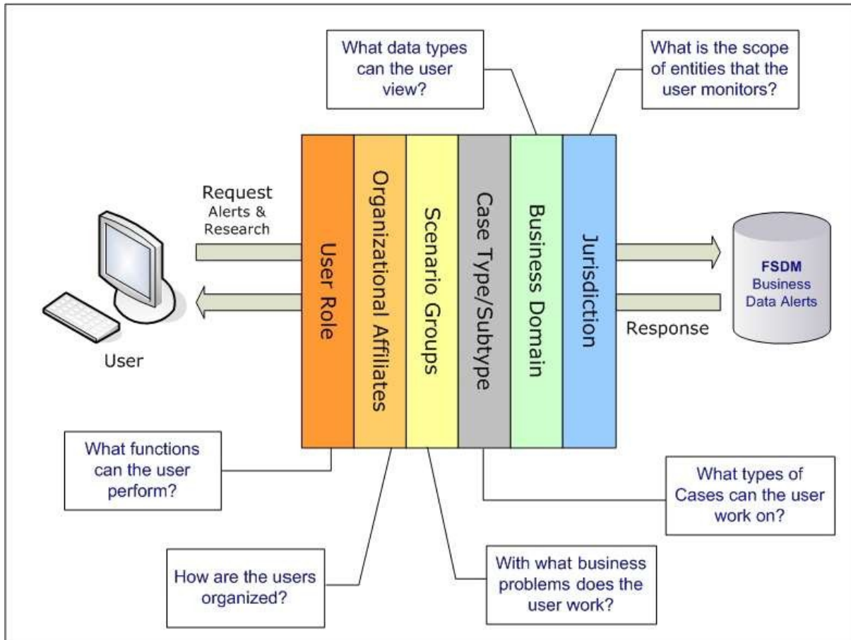
Figure 8. User Authorization Model
