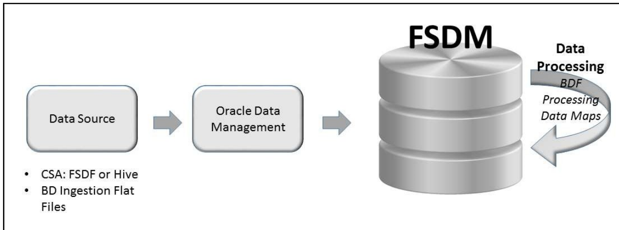
Figure 11. Data Loading and Processing Flow Overview
