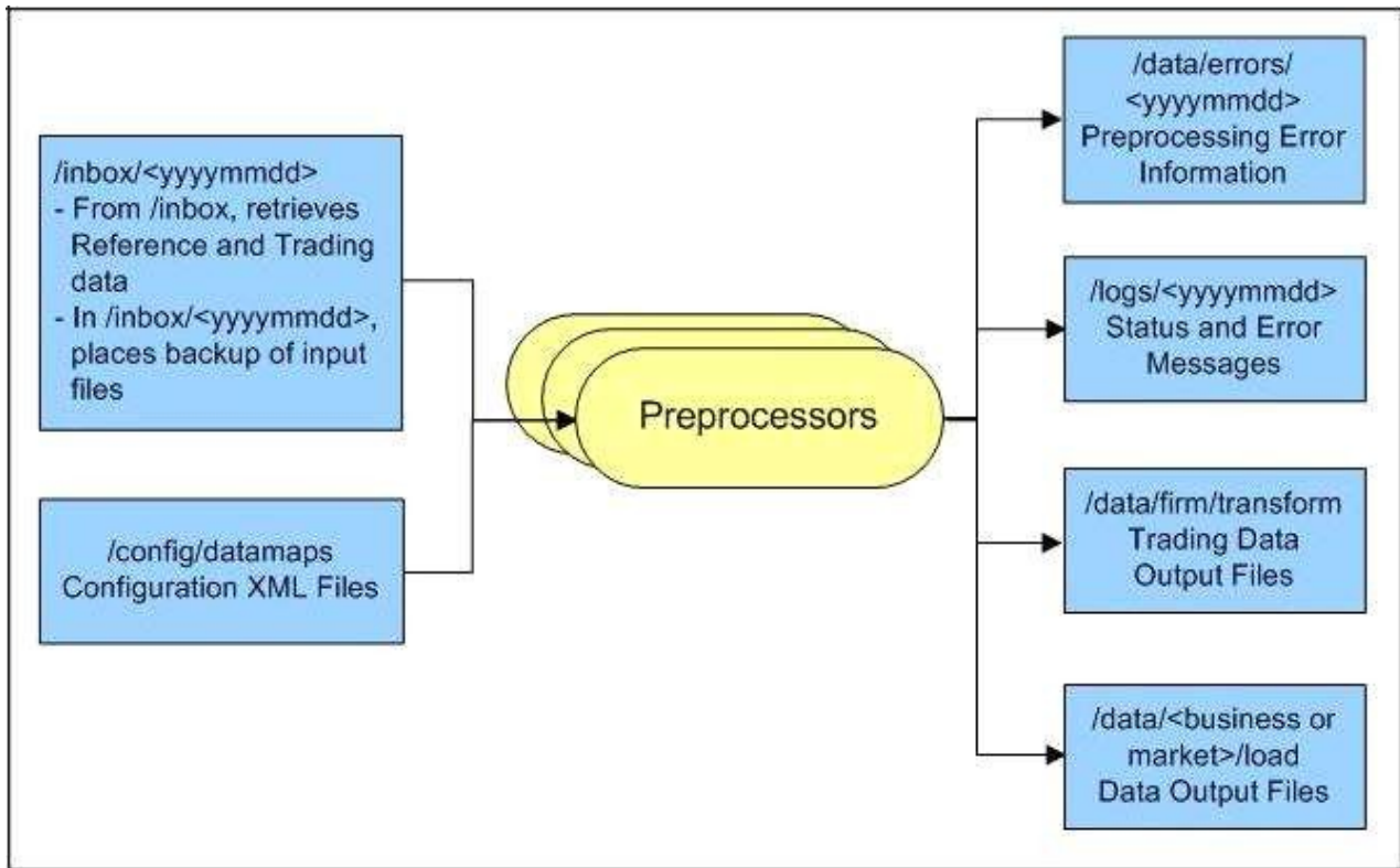
Figure 16. Input and Output Directories
