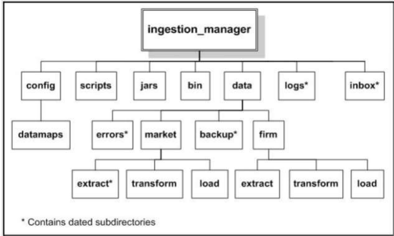
Figure 38. Data Management Subsystem Directory Structure
