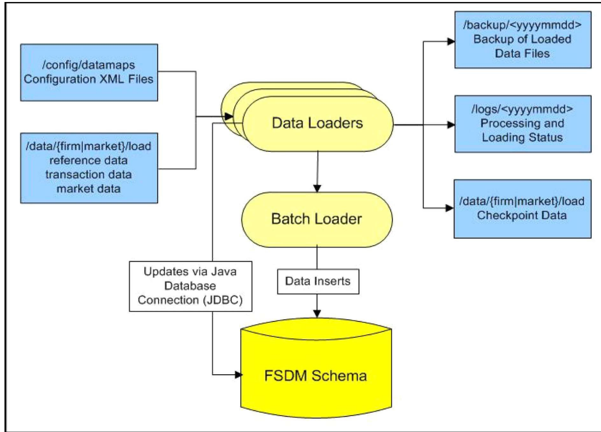
Figure 17. TCS Data Loading Process
