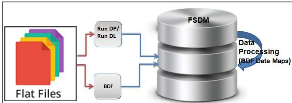
Figure 15. Data Loading Flow Using Flat File Interface
