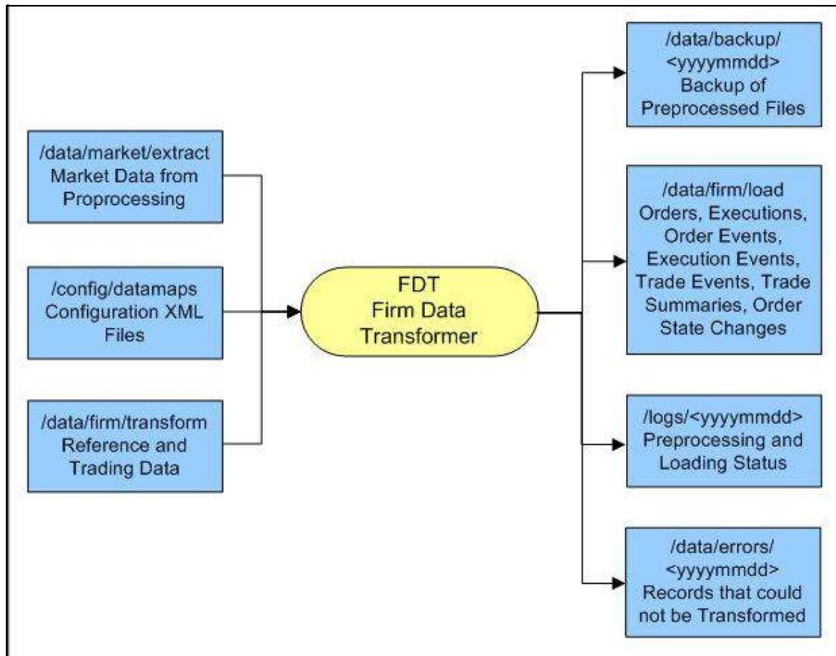
Figure 18. Firm Data Transformer (FDT) Processing
