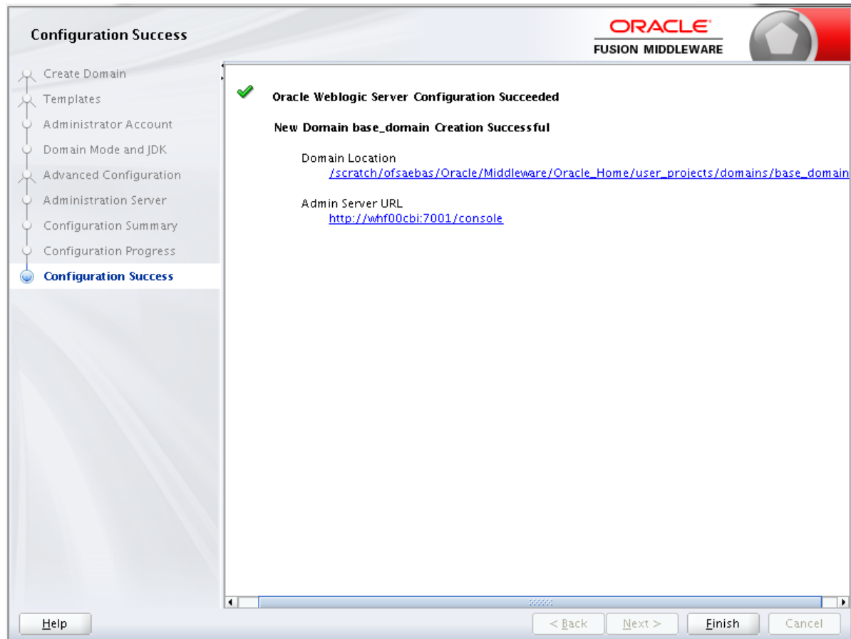
Figure 7–5 Configuration Success
