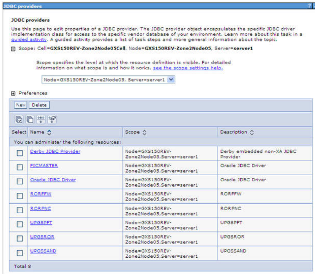
Figure 7–6 JDBC Providers
