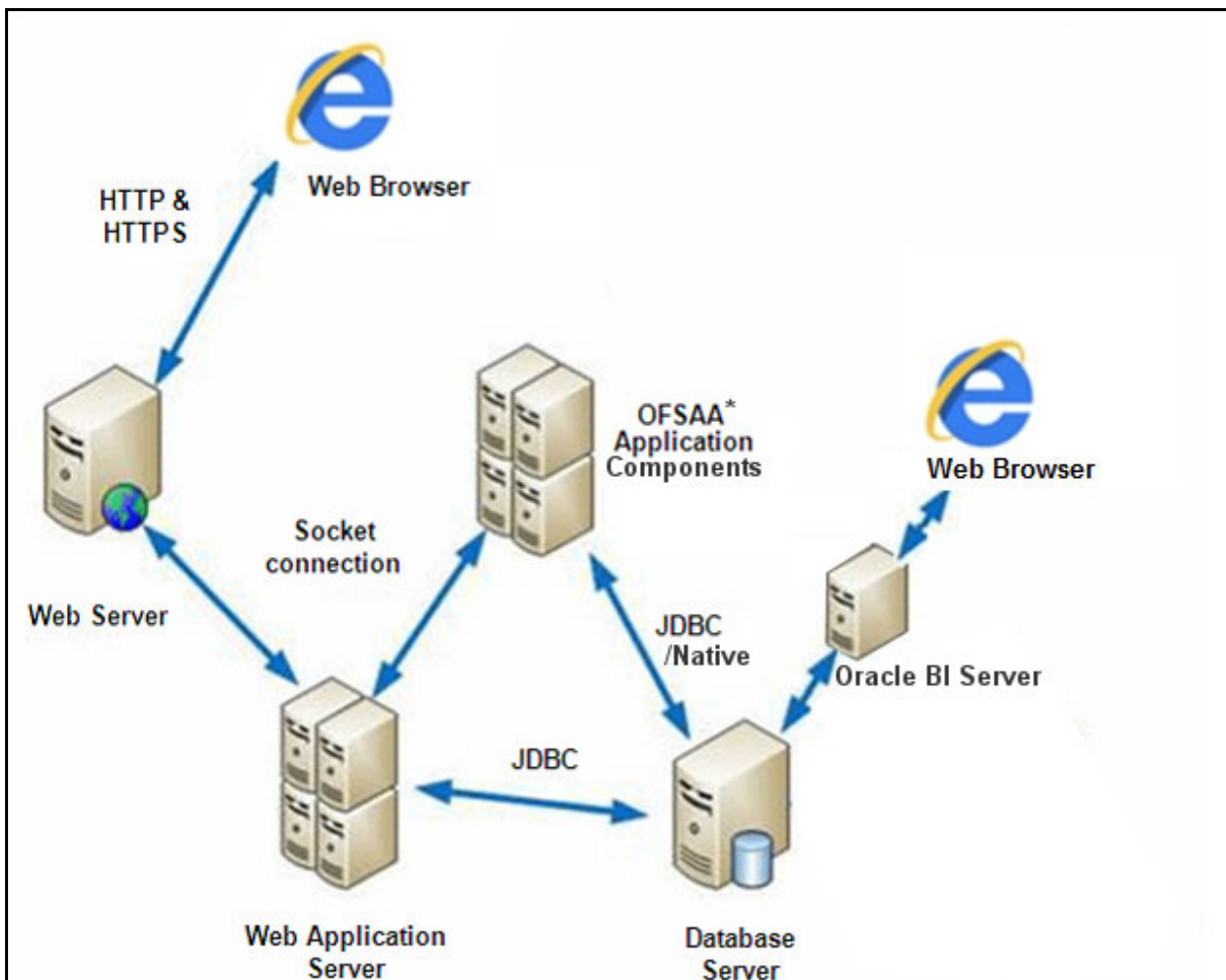
Figure 2-2 Deployment Topology
