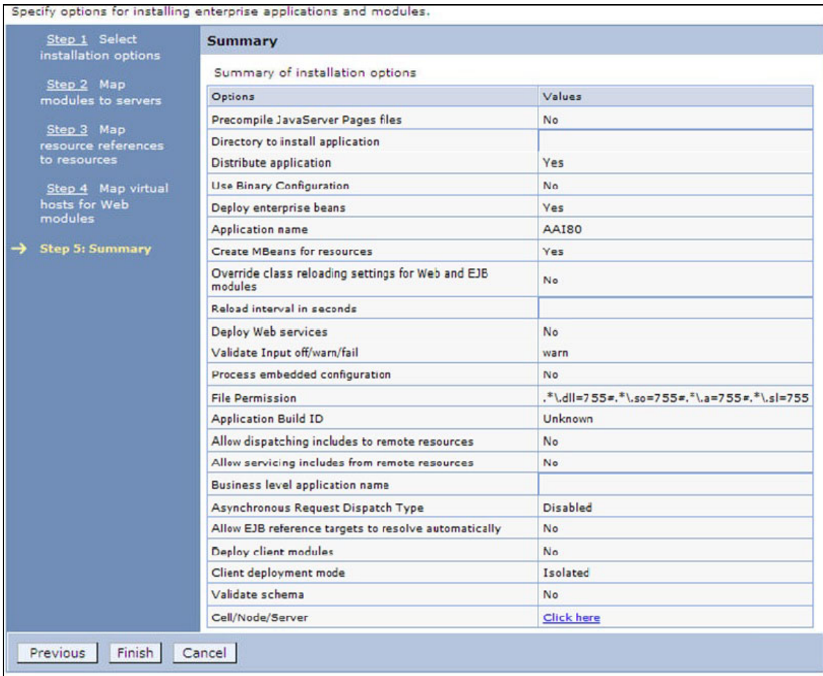
Figure C-10 Summary
