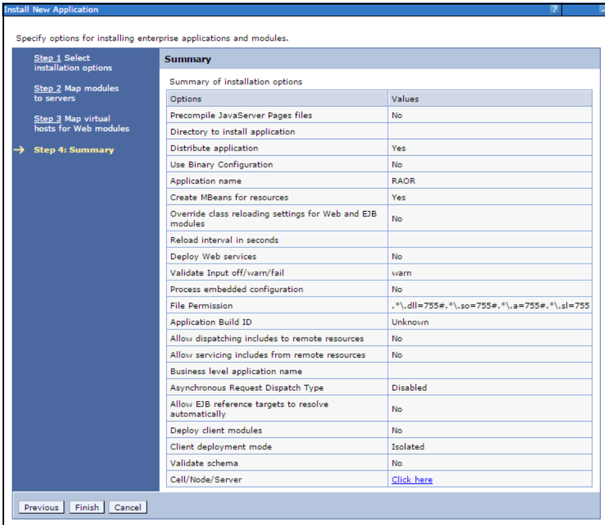
Figure 6–16 Summary page
