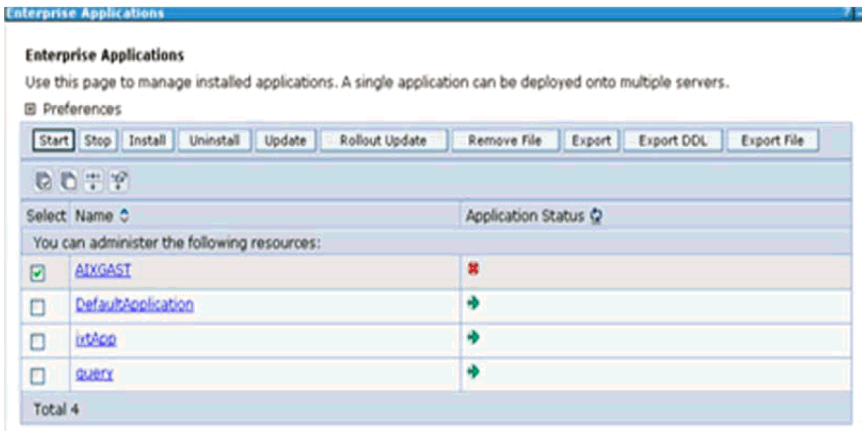
Figure 7–2 Enterprise Applications
