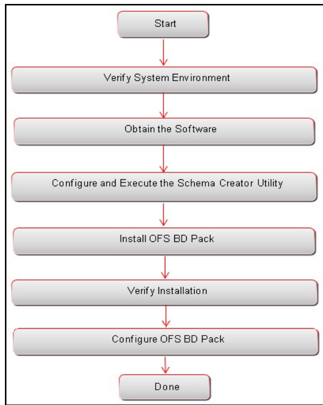
Figure 2–1 Installation Overview
