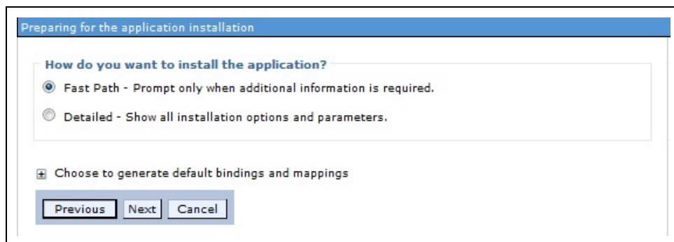
Figure 6–12 Installation Options
