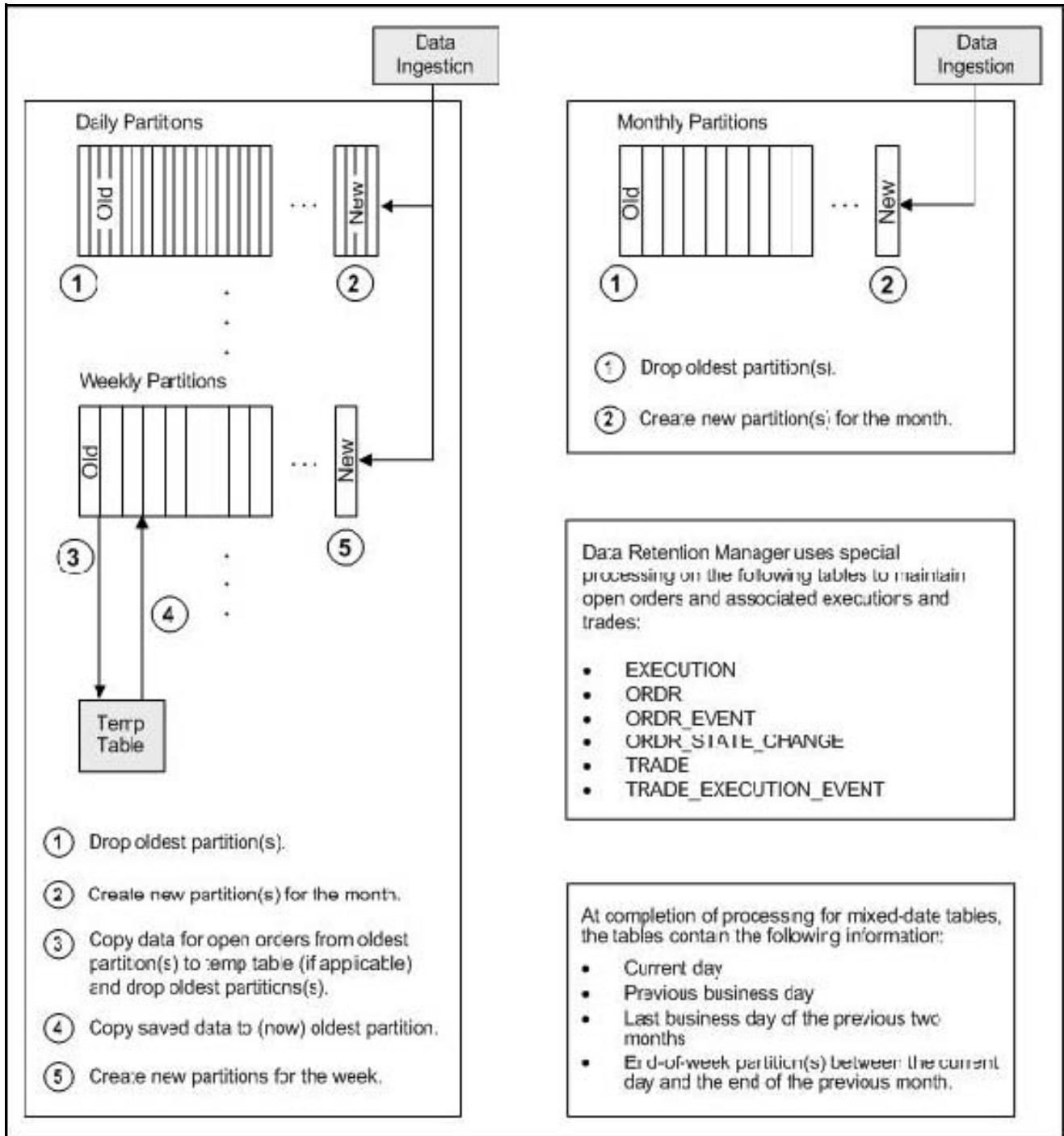
Figure 25: Database Partitioning Process
