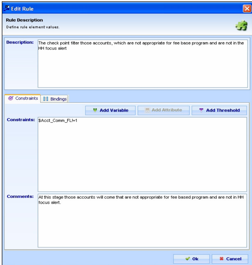
Figure 52: Edit Rule Dialog Box—Checkpoint
