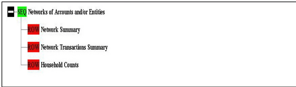
Figure 19: Sequence Scenario Editor-Pattern Editor Area
