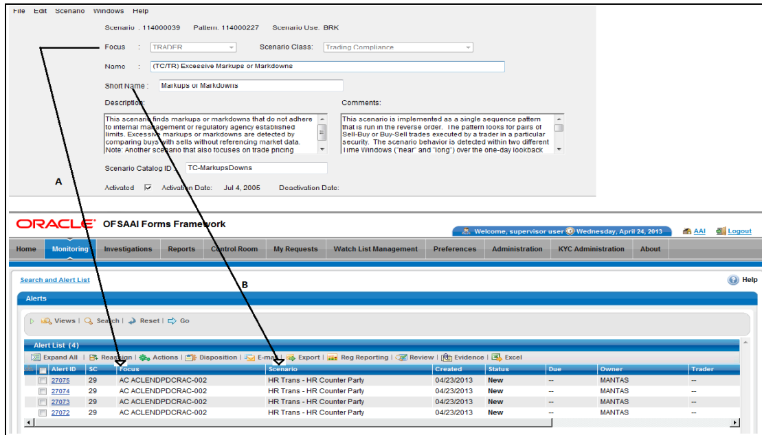
Figure 69: UI Mapping Sample- Scenario Editor to Alert List
