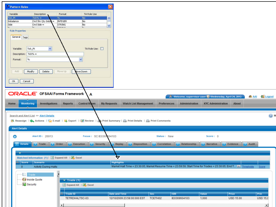
Figure 71: UI Mapping Sample- Pattern Role Editor to Alert List
