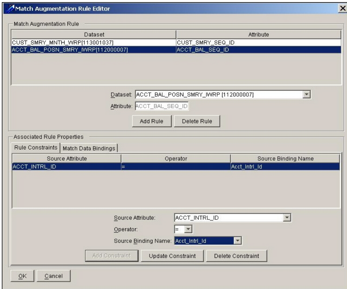
Figure 62: Match Augmentation Rule Editor Dialog Box
