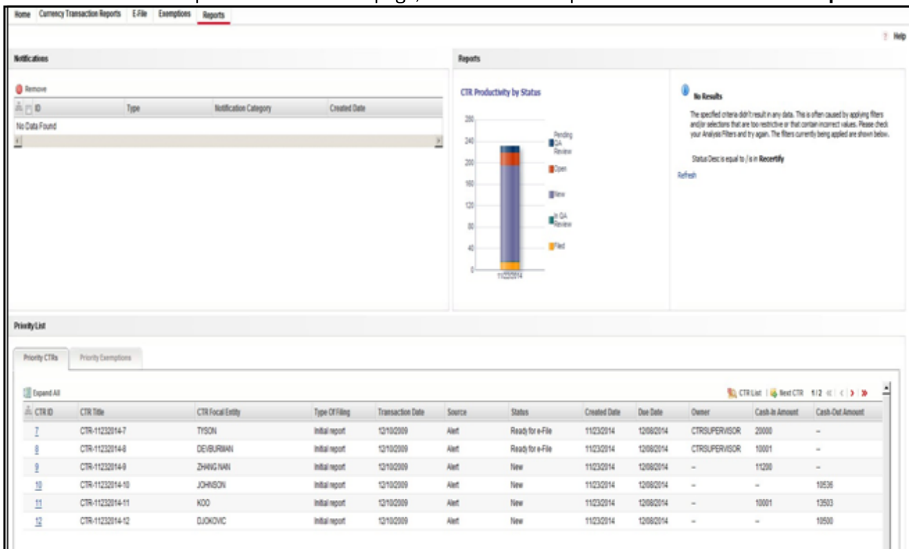
Figure 1: Accessing Reports
