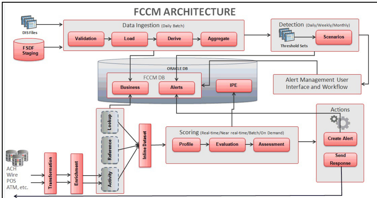
Figure 1: OFSBD Architecture
