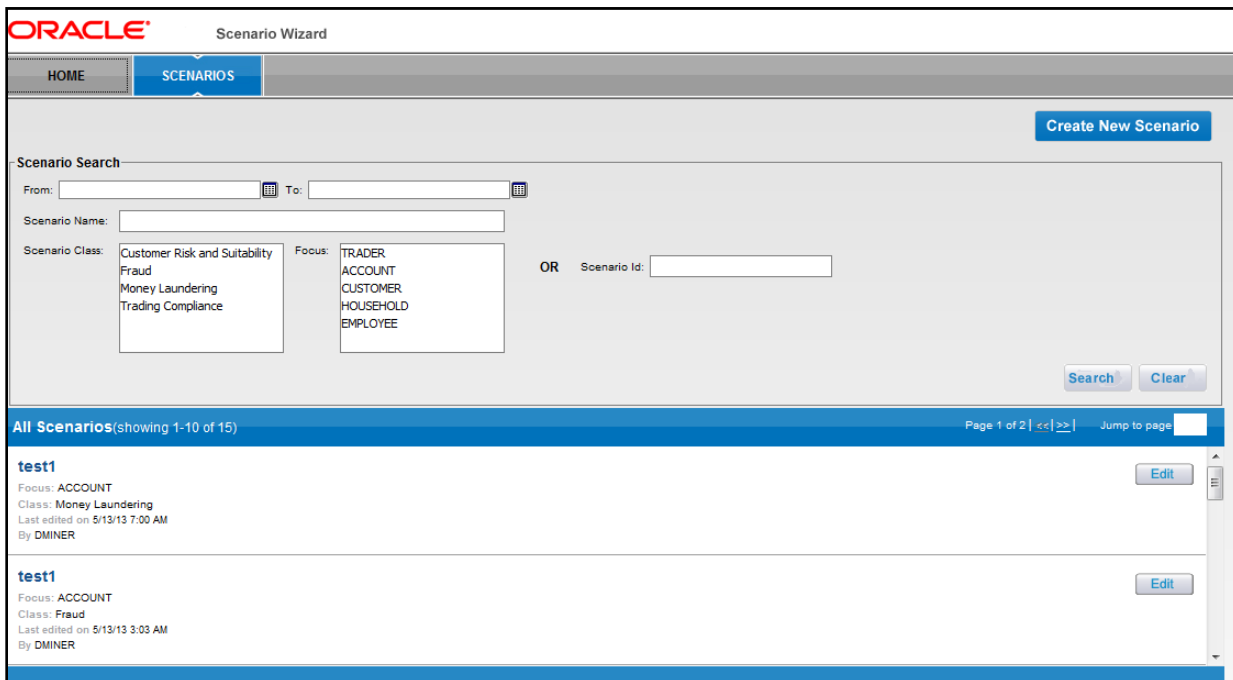
Figure 9. Scenario Page
