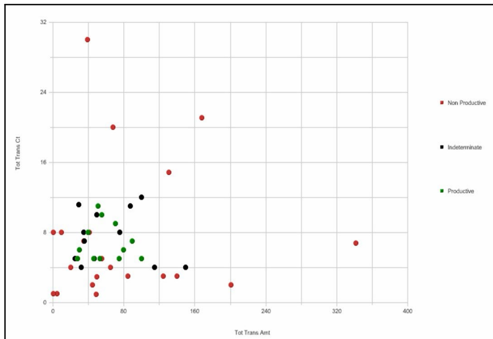
Figure 61. Scatter Graph
