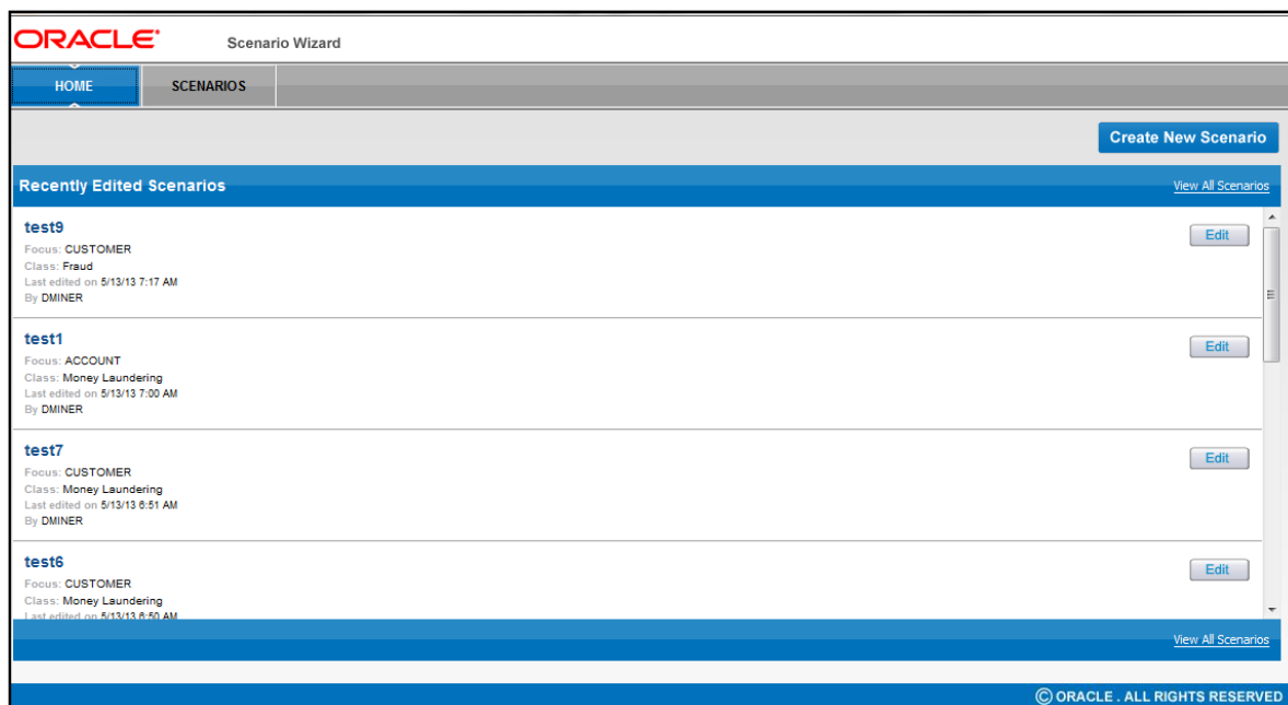
Figure 8. Home Page
