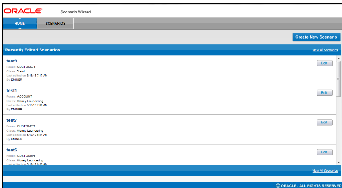
Figure 8. Home Page
