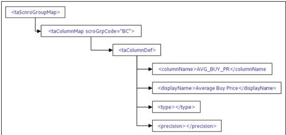
Figure 4: TA Column Map
