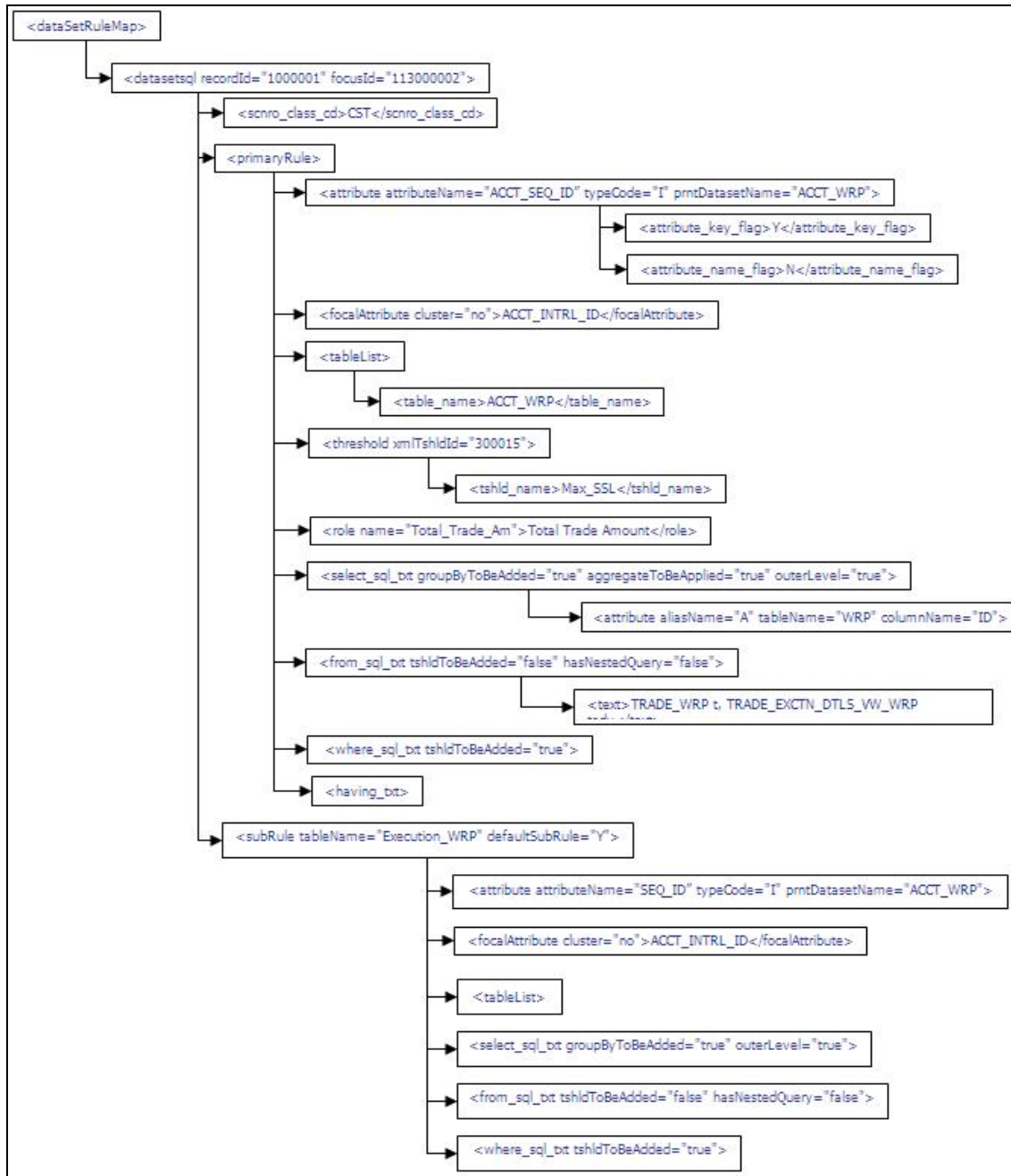
Figure 5: Data Set Rule Map
