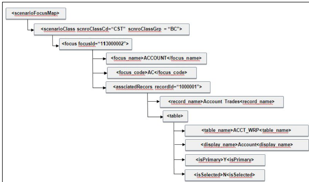
Figure 2: Scenario Focus Mapping
