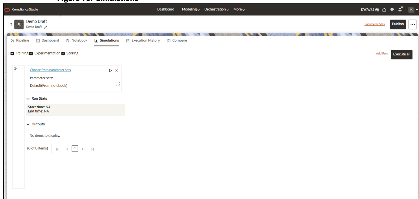
Figure 96: Simulations
