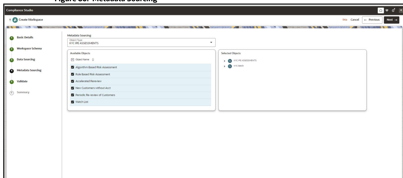
Figure 86: Metadata Sourcing
