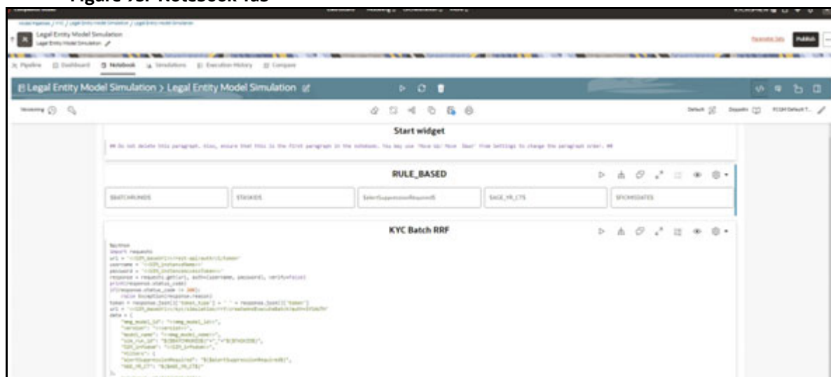
Figure 95: Notebook Tab
