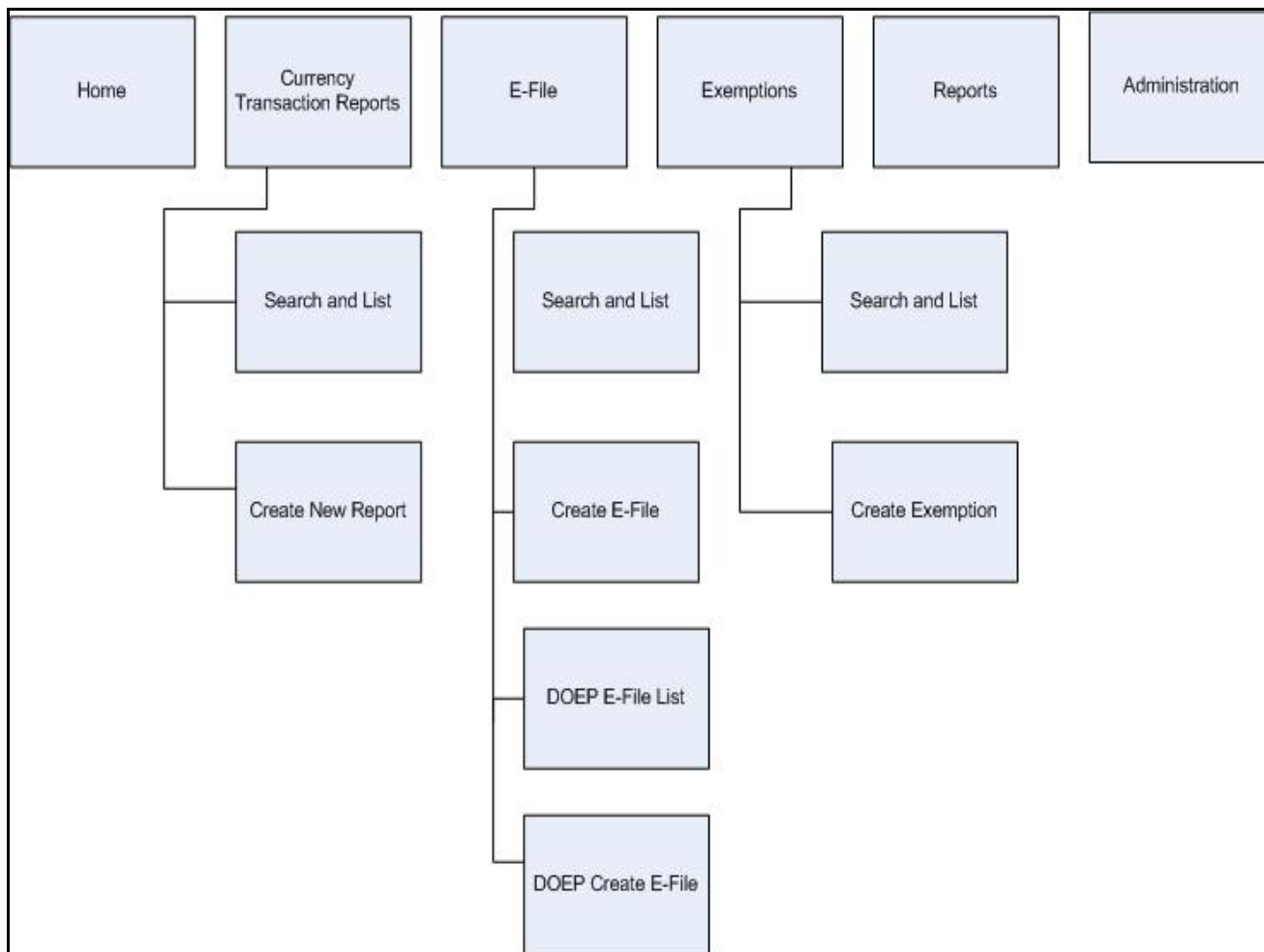
Figure 4: CTRs Menus
