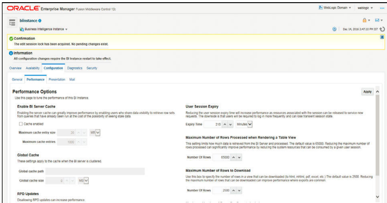
Figure 5–1 Disabling the Cache Feature in OBIEE Server (12.2.1.3.0)
