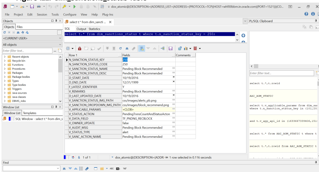
Figure 122: dim_Sanctions_status Table
