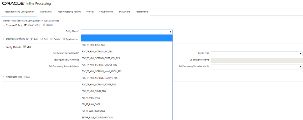
Figure 93: Entities List
