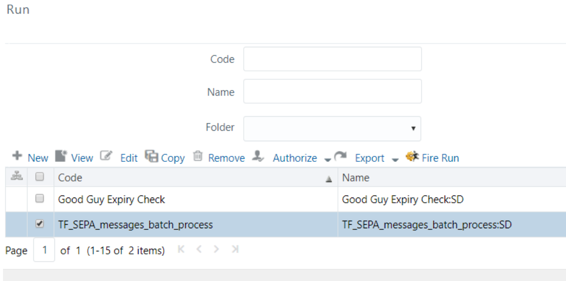
Figure 71: Run Page
