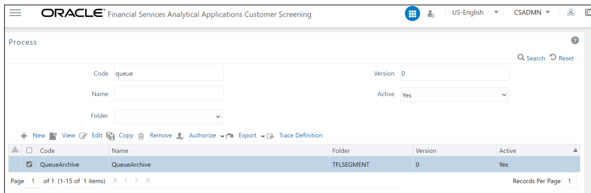
Figure 23: Process Page
