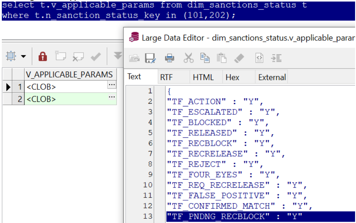
Figure 123: Applicable Params
