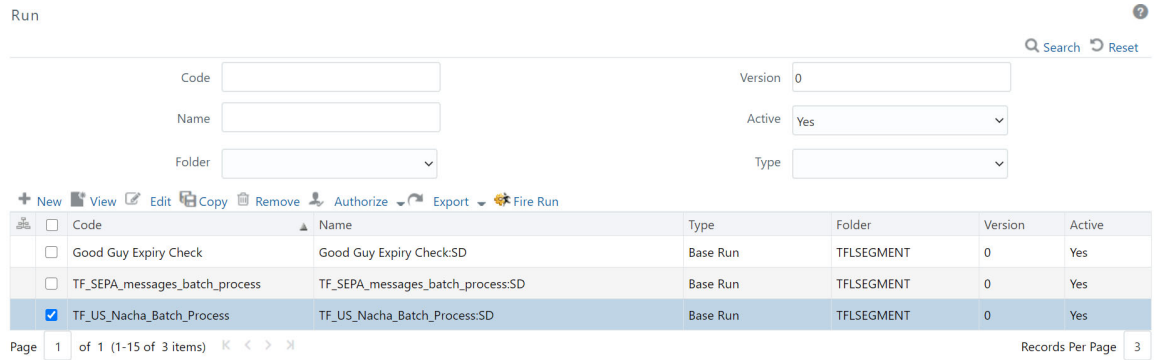
Figure 77: Run Page
