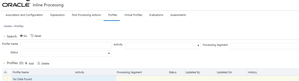
Figure 90: Profiles Menu
