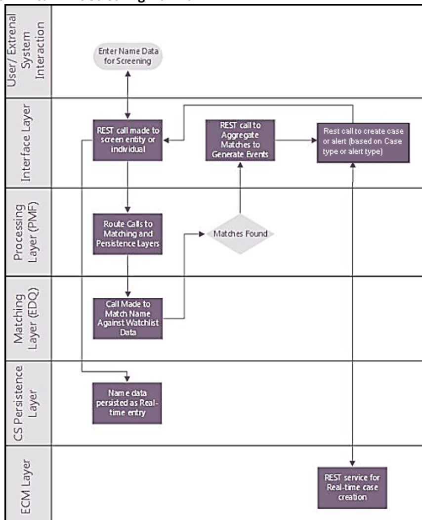
Figure 71: Real-Time Screening Workflow
