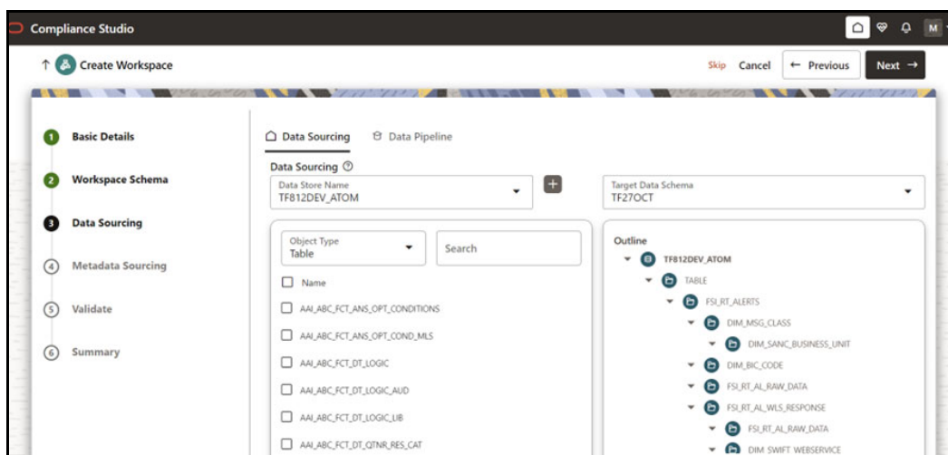
Figure 122: Data Sourcing
