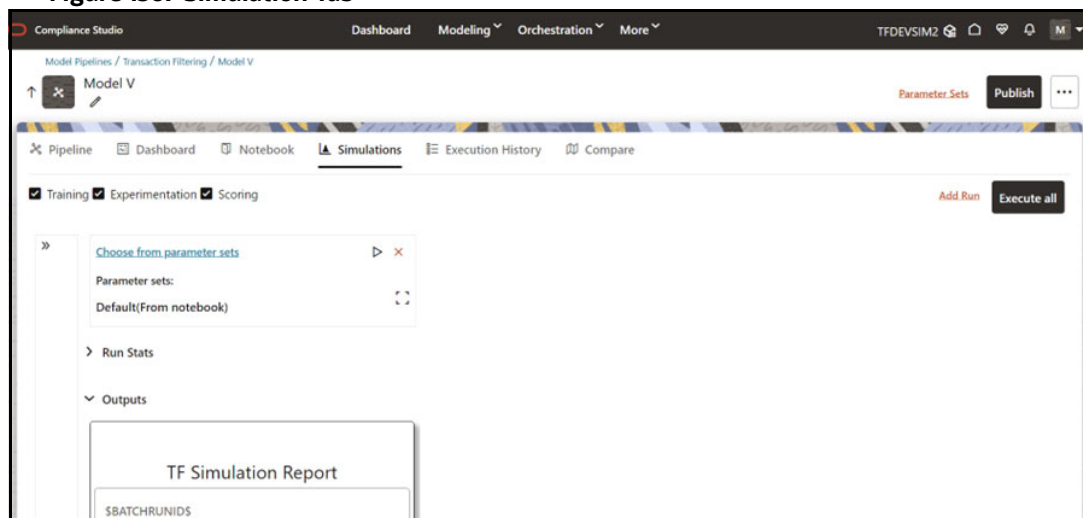
Figure 136: Simulation Tab
