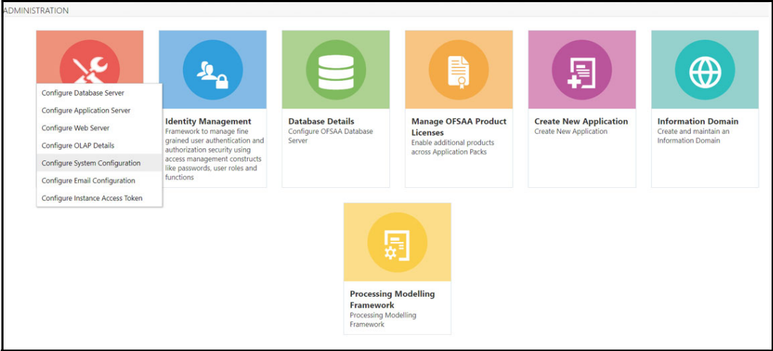
Figure 5: Administration Page
