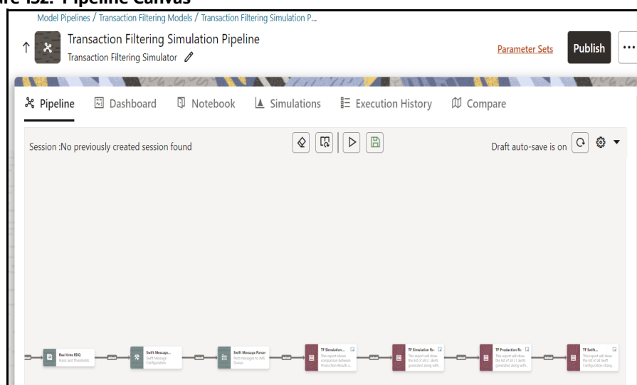
Figure 132: Pipeline Canvas
