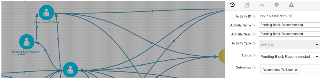
Figure 147: Activity Statuses
