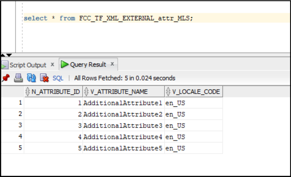
Figure 69: Example 2
