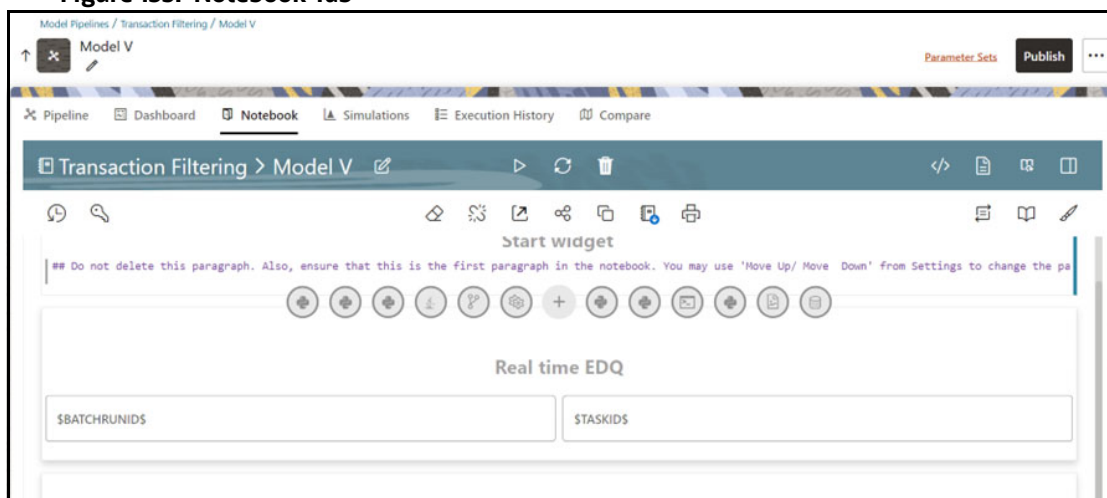
Figure 135: Notebook Tab
