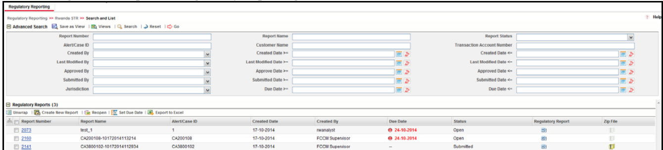
Figure 11. Advanced Search
