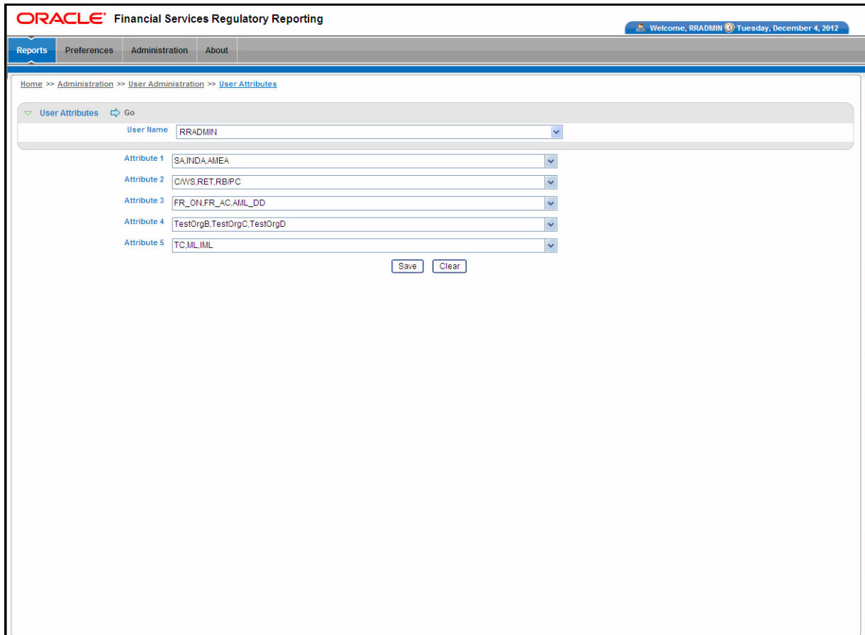
Figure 37. User Administration
