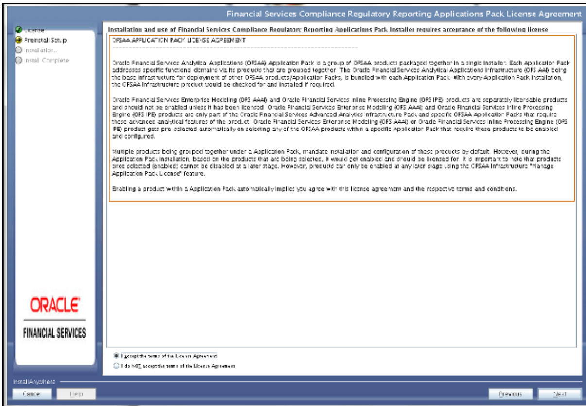
Figure 4-5 License Agreement
