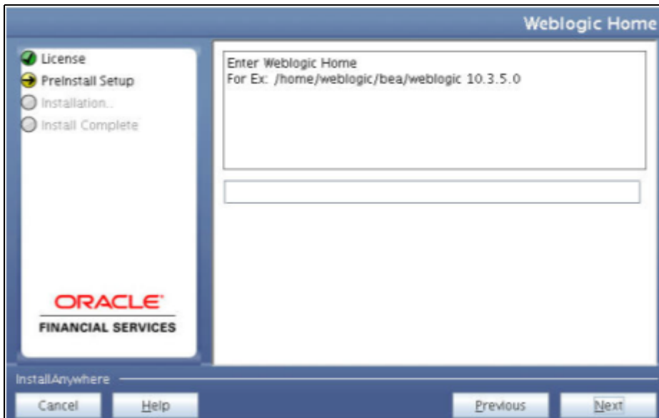
Figure 4–17 Weblogic Home
