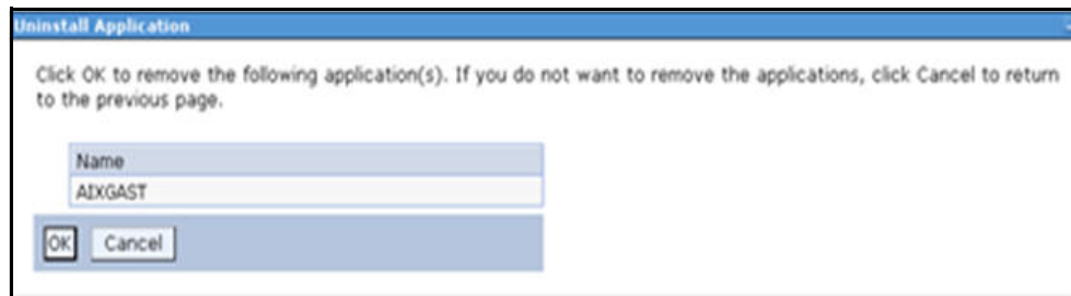
Figure 5–61 Uninstall Application
