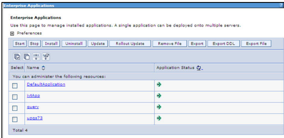
Figure 5–60 Enterprise Applications
