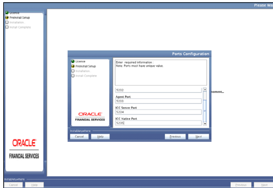
Figure 4-22 Ports Configuration
