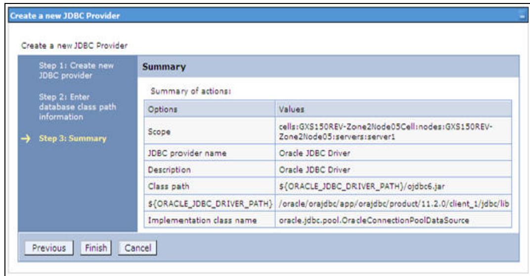
Figure 5–15 Summary
