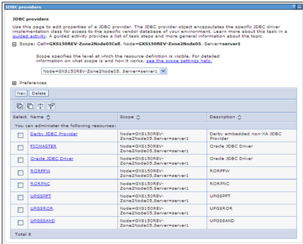
Figure 5–12 JDBC Providers
