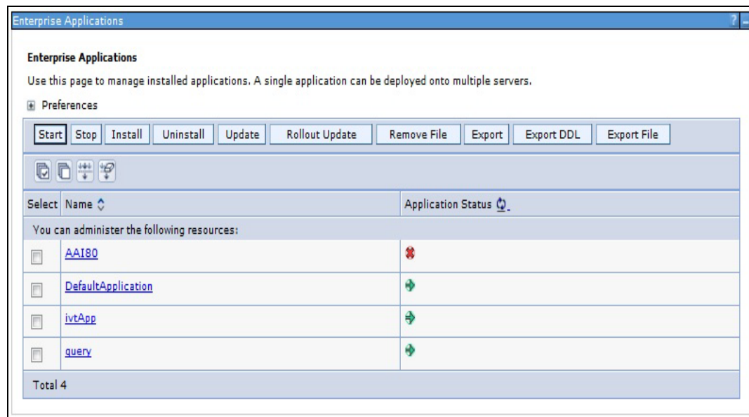
Figure 5-48 Enterprise Applications
