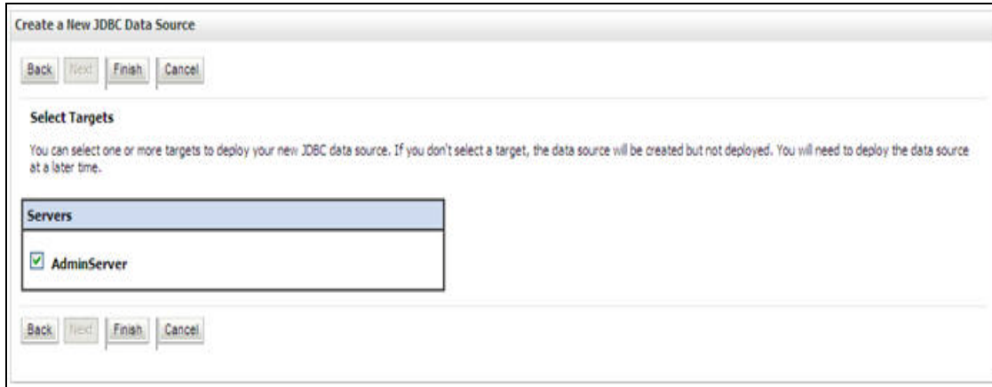
Figure 5–30 Select Targets
