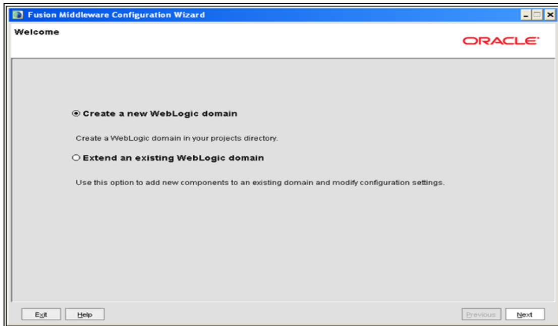
Figure 5–3 Welcome
