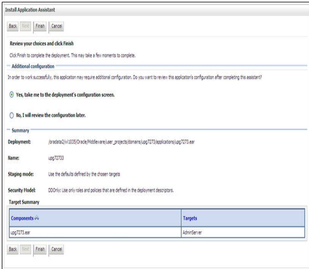
Figure 5–53 Deployment Summary
