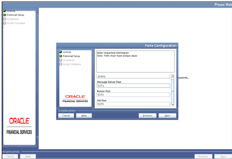
Figure 4–23 Ports Configuration
