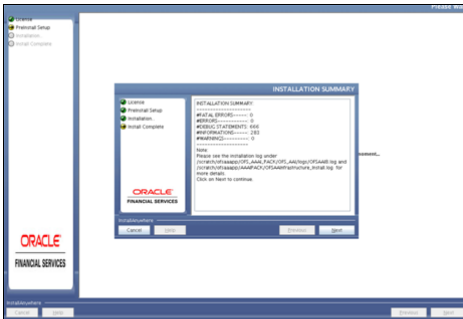
Figure 4–29 Installation Summary
