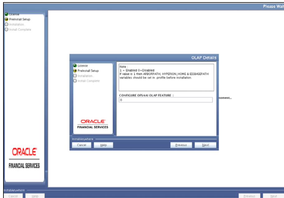
Figure 4–19 OLAP Details
