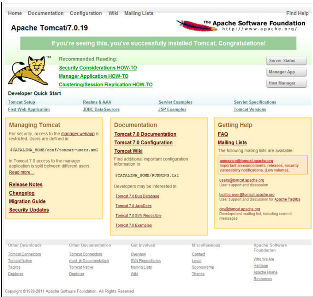
Figure 5-57 Tomcat home
