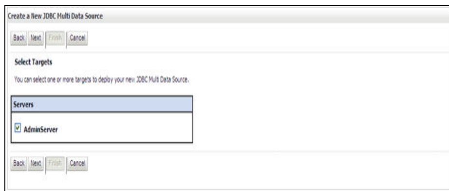
Figure 5–35 Select Targets
