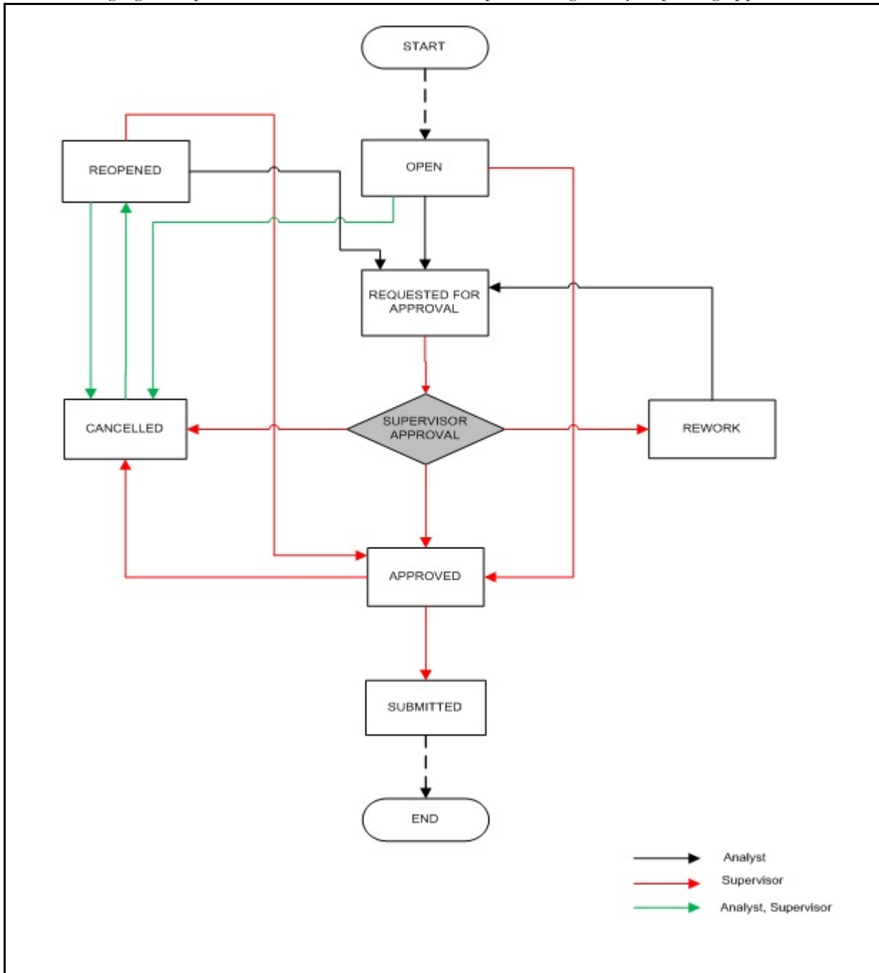
Figure 3. Compliance Regulatory Reporting workflow for Analyst and Supervisor
