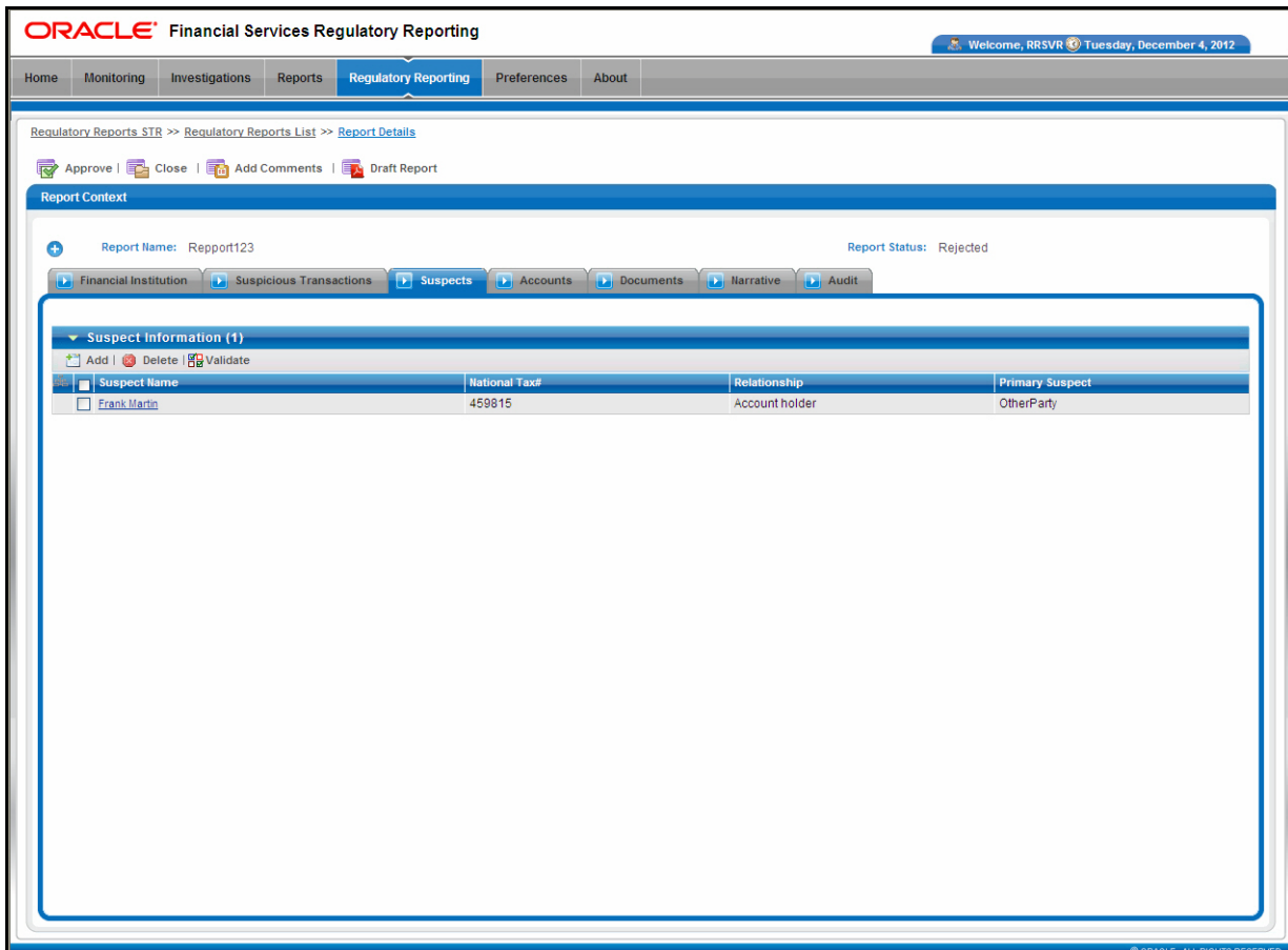
Figure 18. Suspects Tab
