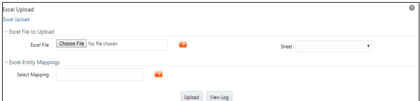
Figure 2: Uploading Excel
