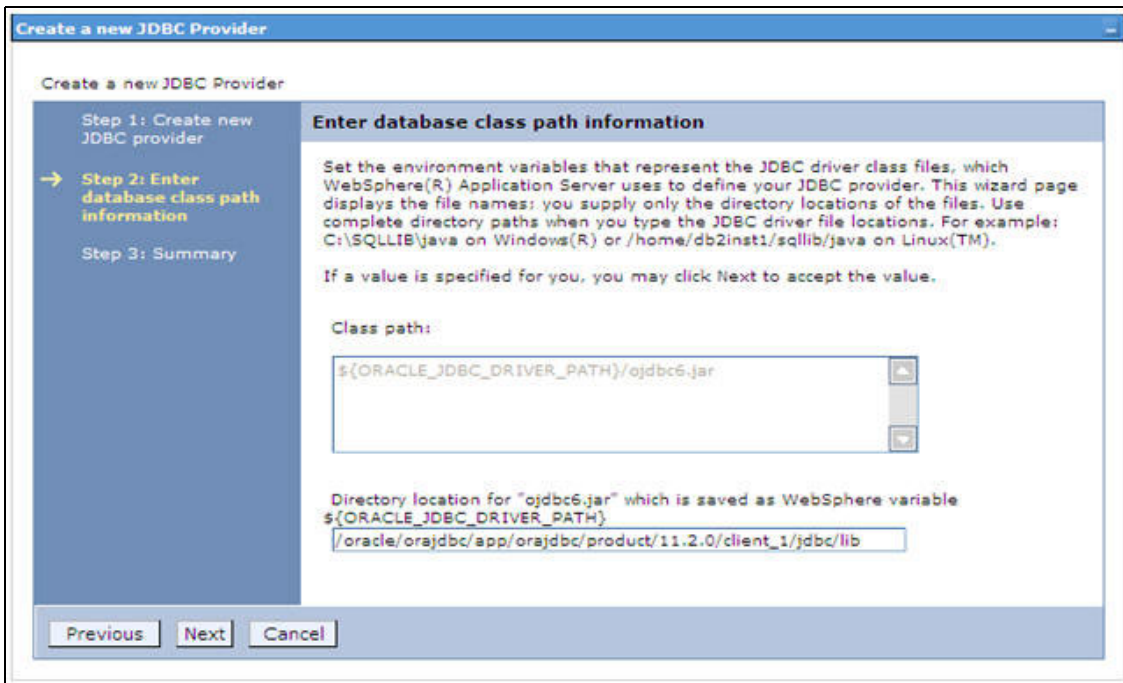
Figure 28: Enter database class path information
