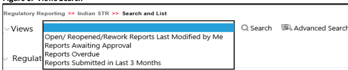
Figure 6: Views Search
