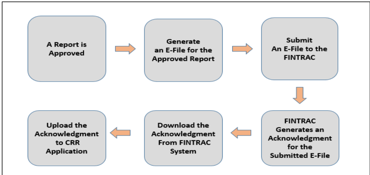
Figure 34: E-Filing Workflow
