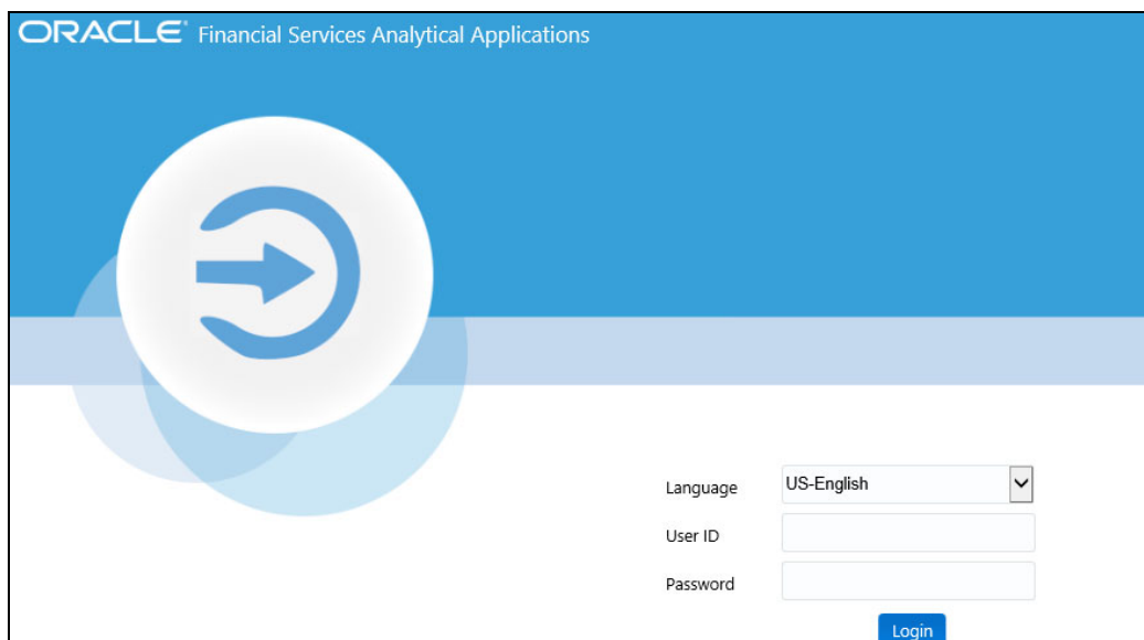
Figure 2: Login Page
