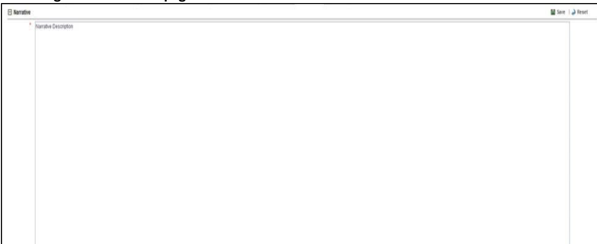
Figure 23: Narrative page
