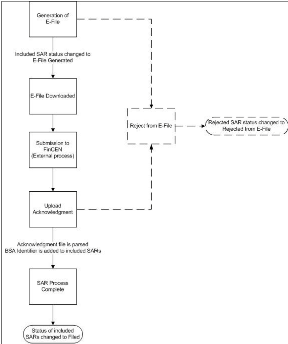
Figure 27: Filing Regulatory Reporting Workflow
