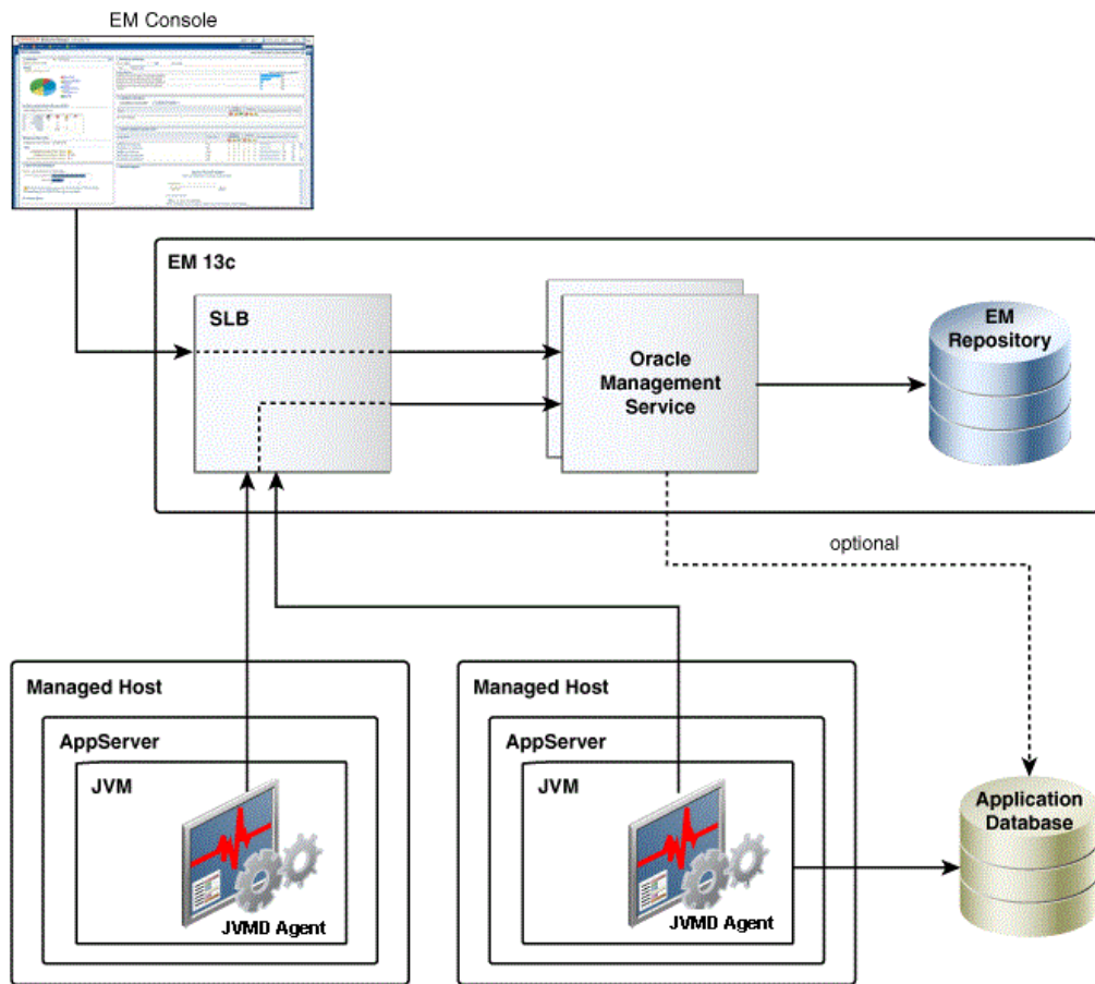
Figure 15-1 JVMD Architecture
