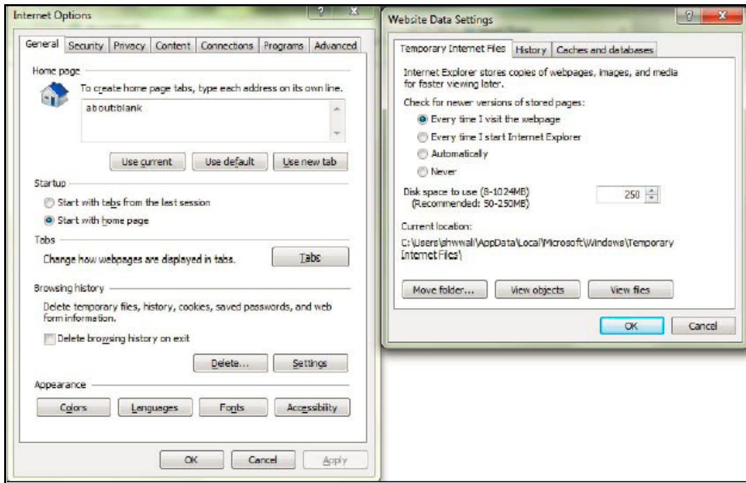
Figure I-1 Internet Options
