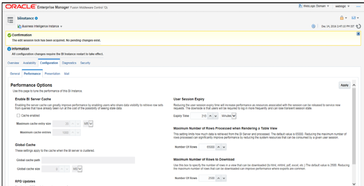
Figure 7–1 Disabling the Cache Feature in OBIEE Server (12.2.1.4.0)
