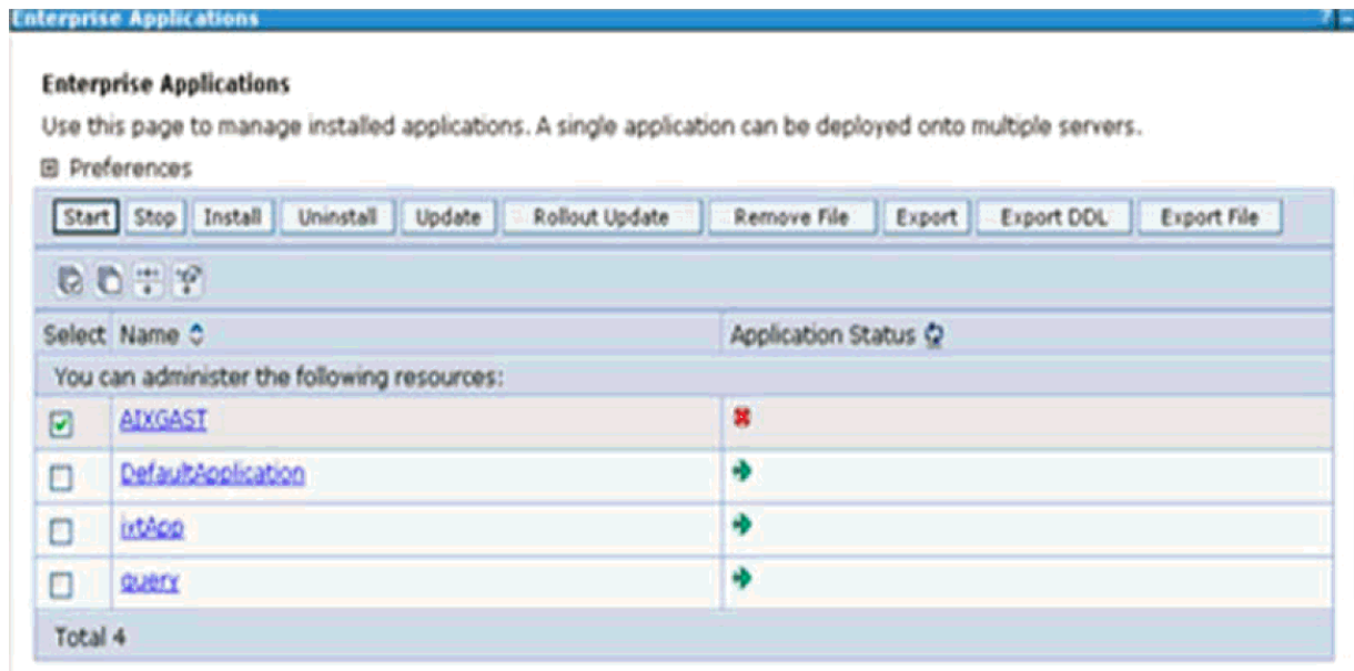
Figure 7-4 Enterprise Applications
