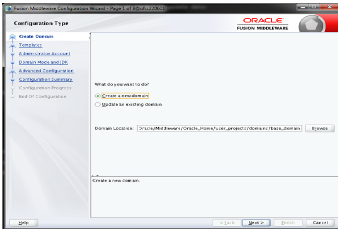
Figure 7-5 Configuration Type
