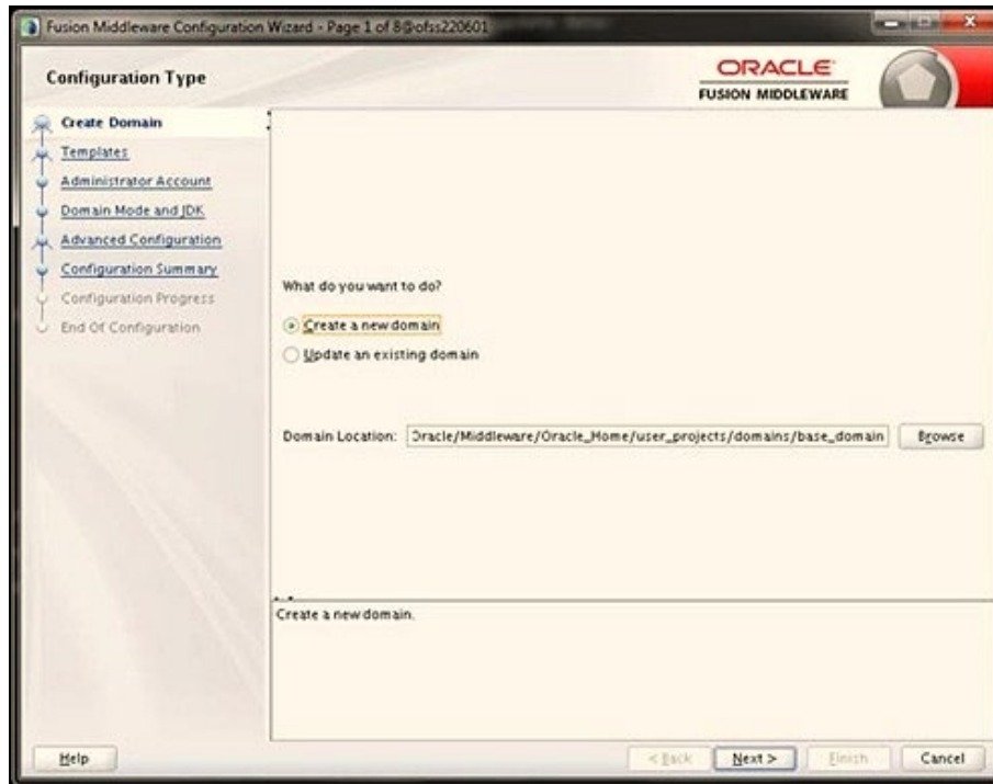
Figure 9: Configuration Type
