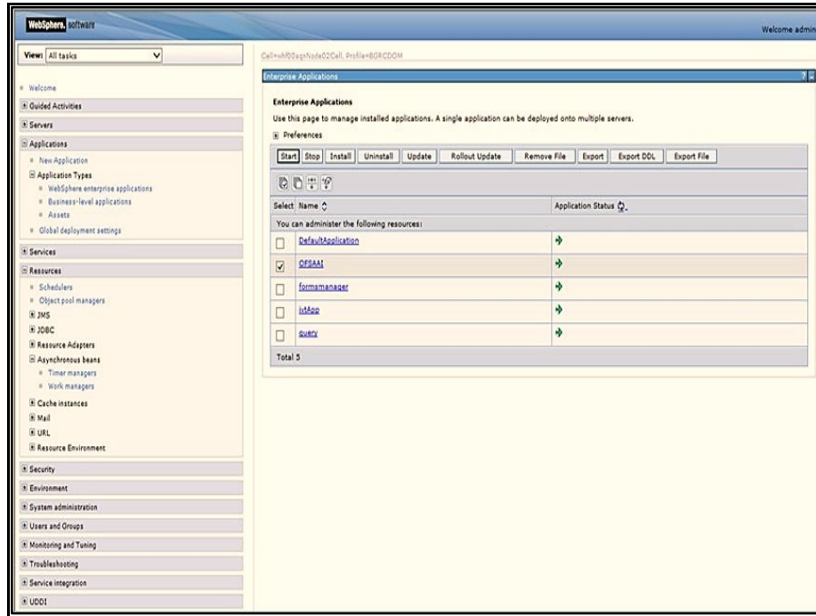
Figure 7: Enterprise Applications
