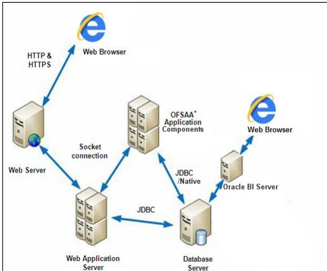
Figure 2–2 Deployment Topology
