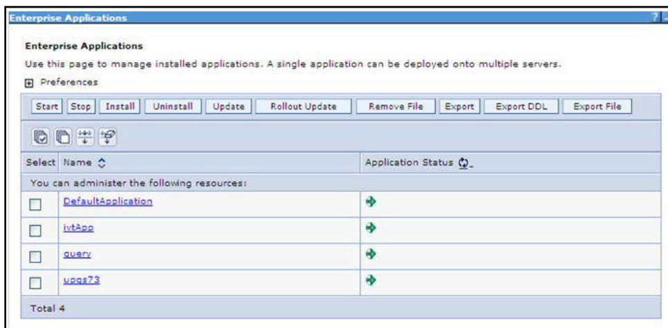
Figure 2–25 Enterprise Applications
