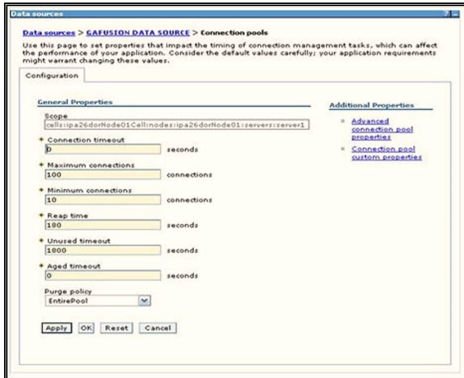
Figure 13: Connection pools
