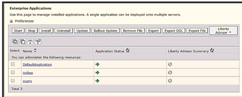
Figure 5: Enterprise Applications
