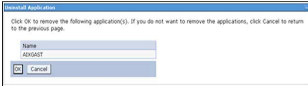
Figure 3–25 Uninstall Application
