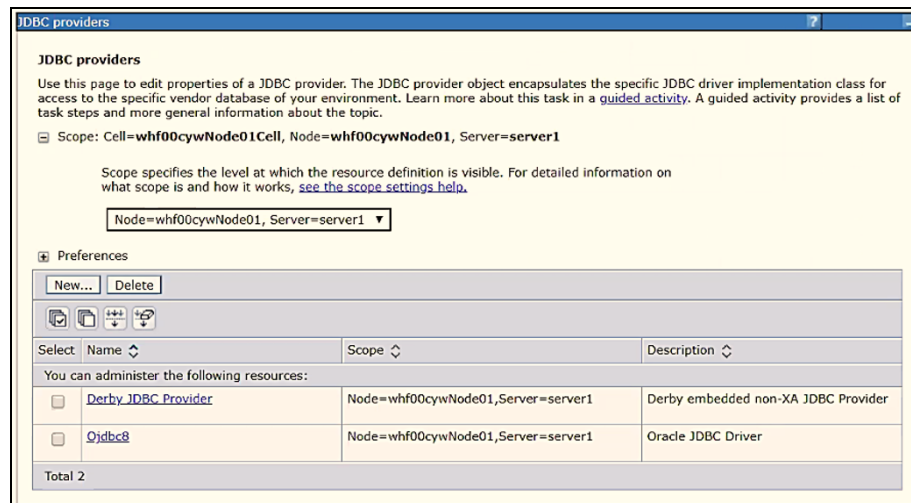
Figure 1: JDBC Providers
