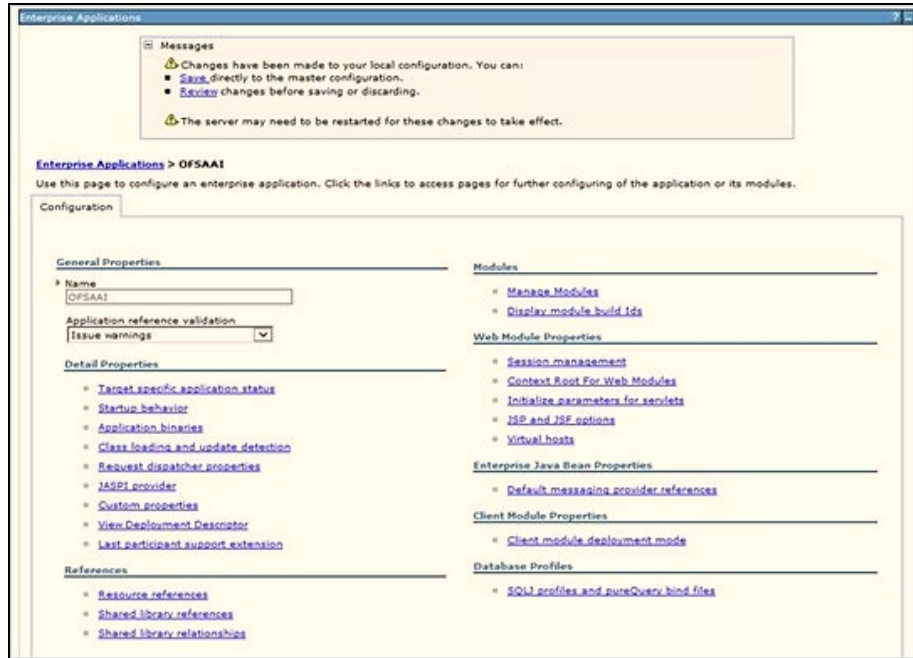
Figure 5: OFSAAI Configuration
