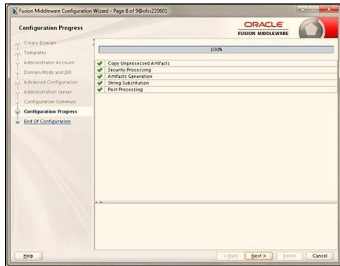
Figure 16: Creating Domain
