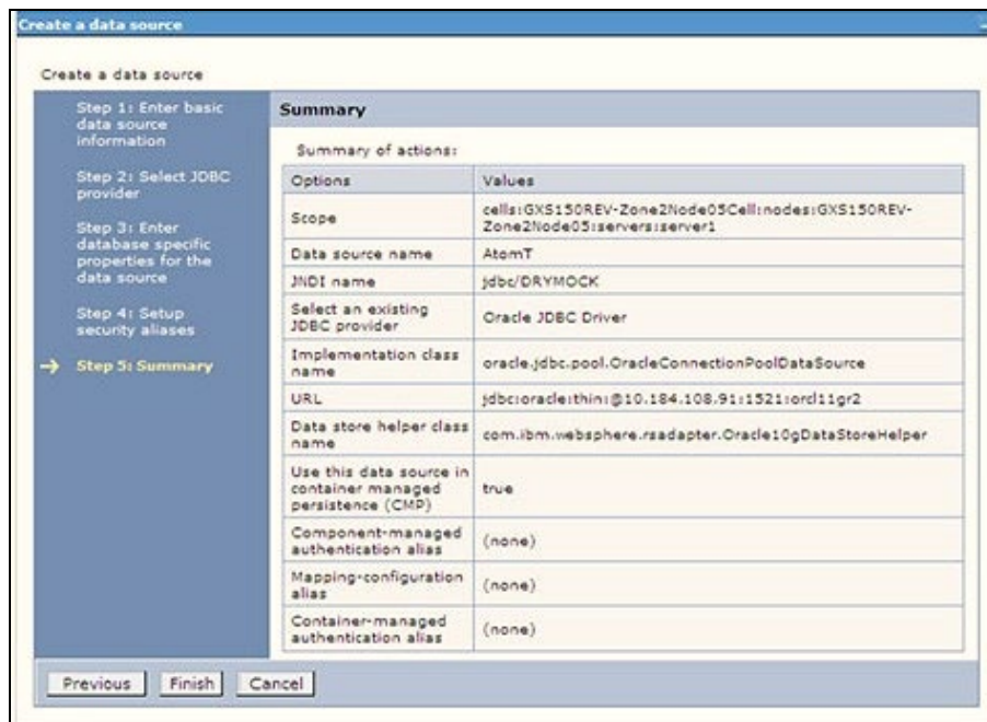
Figure 10: Summary
