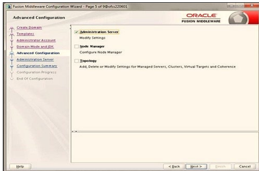
Figure 13: Advanced Configuration
