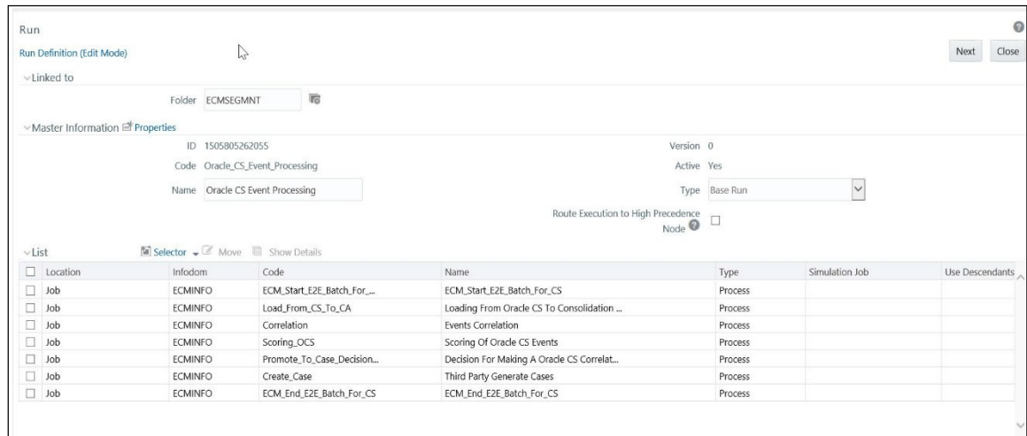
Figure 23: OCS Connector
