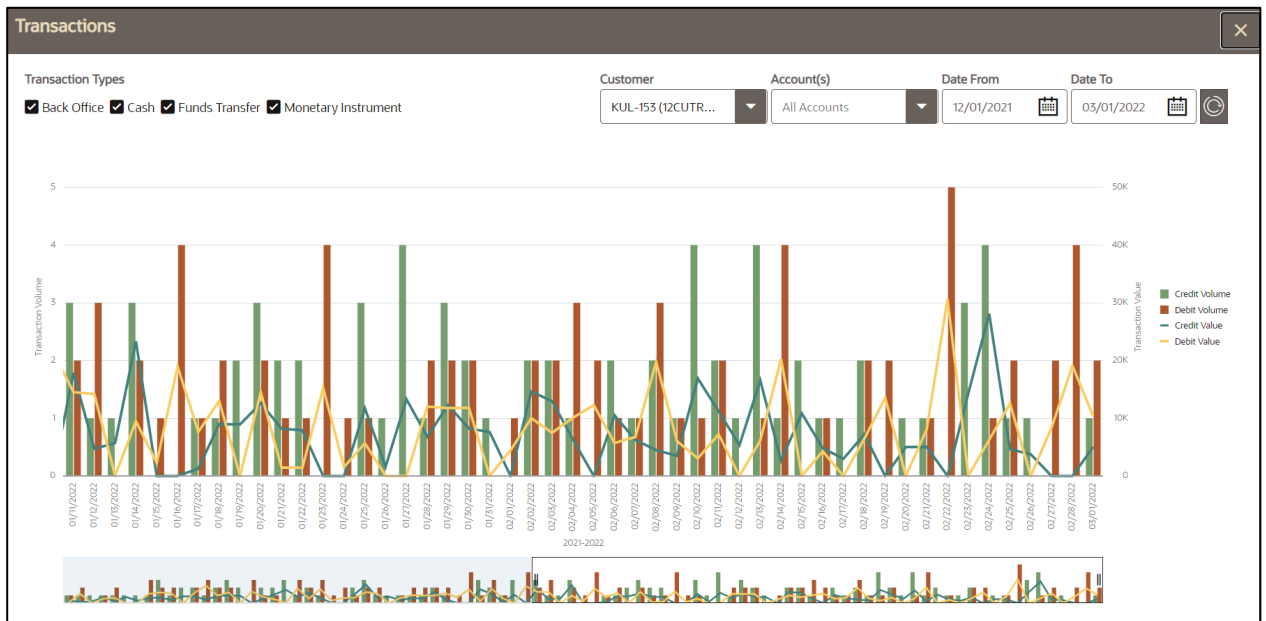
Figure 24: Transaction Chart
