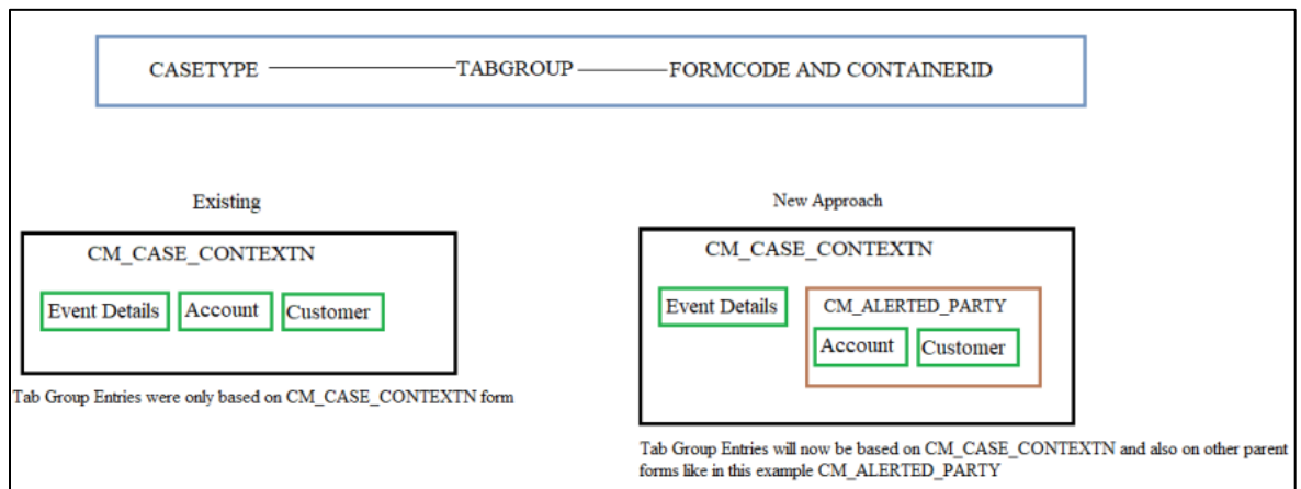
Figure 25: Workflow
