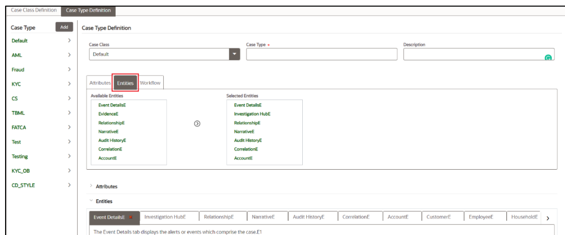
Figure 46: Entities Page
