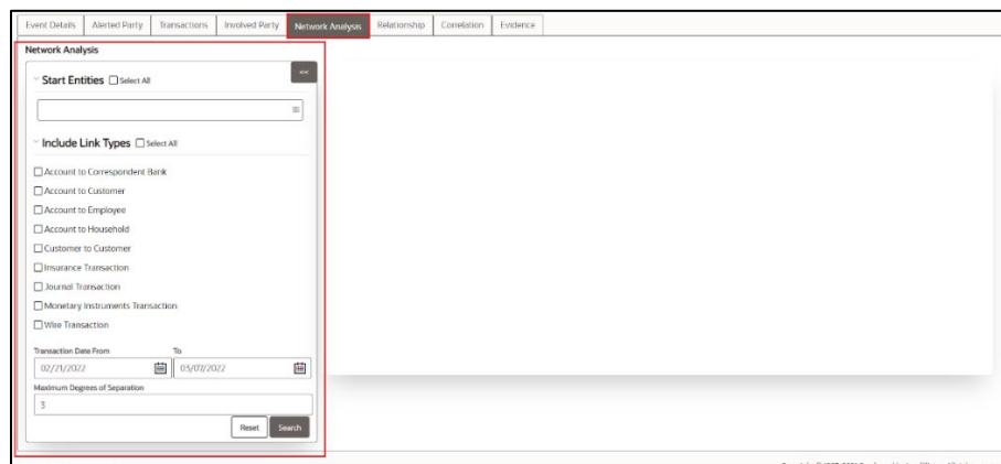
Figure 15: Network Analysis
