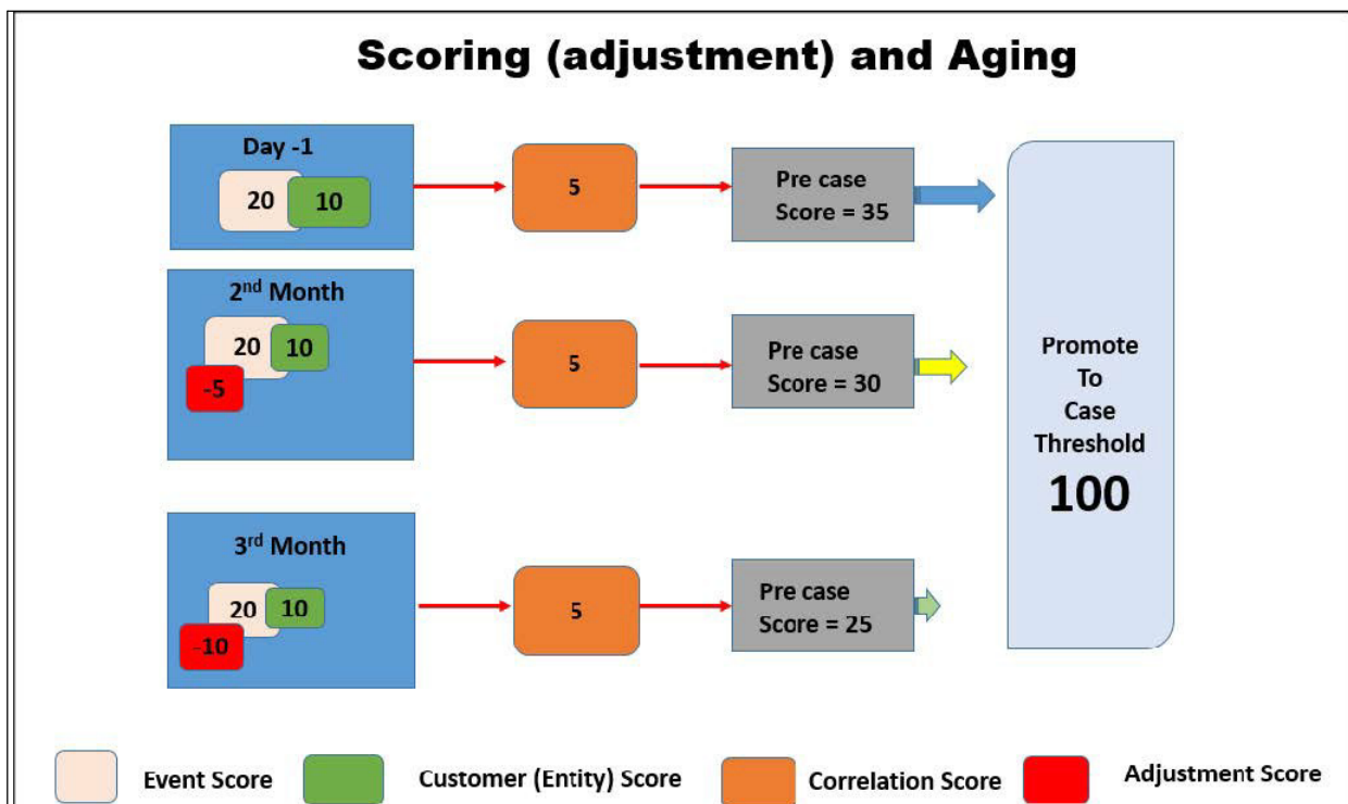
Figure 19: Adjustment Scoring
