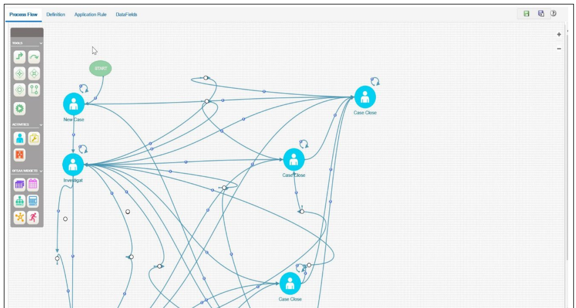
Figure 38: Editing Workflow
