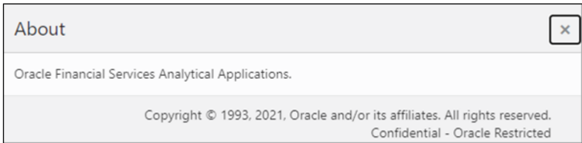
Figure 7: Copyright Information
