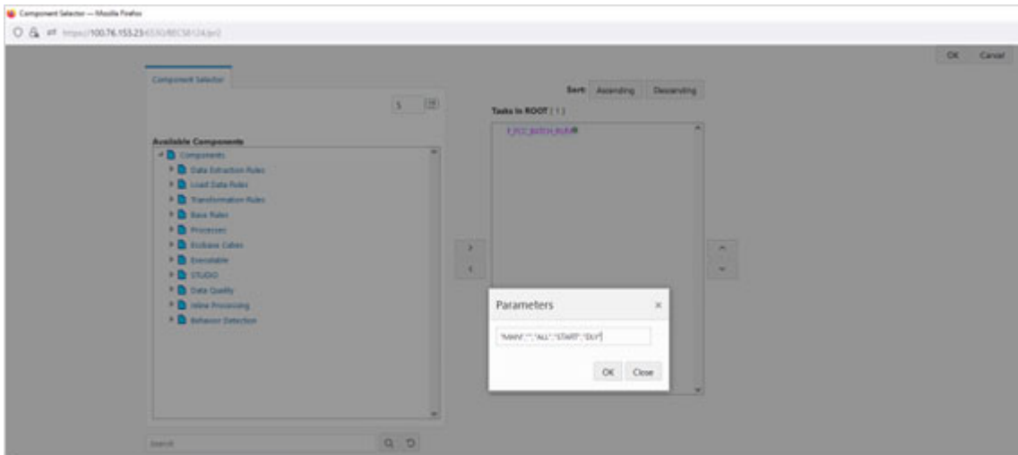
Figure 23: Parameters
