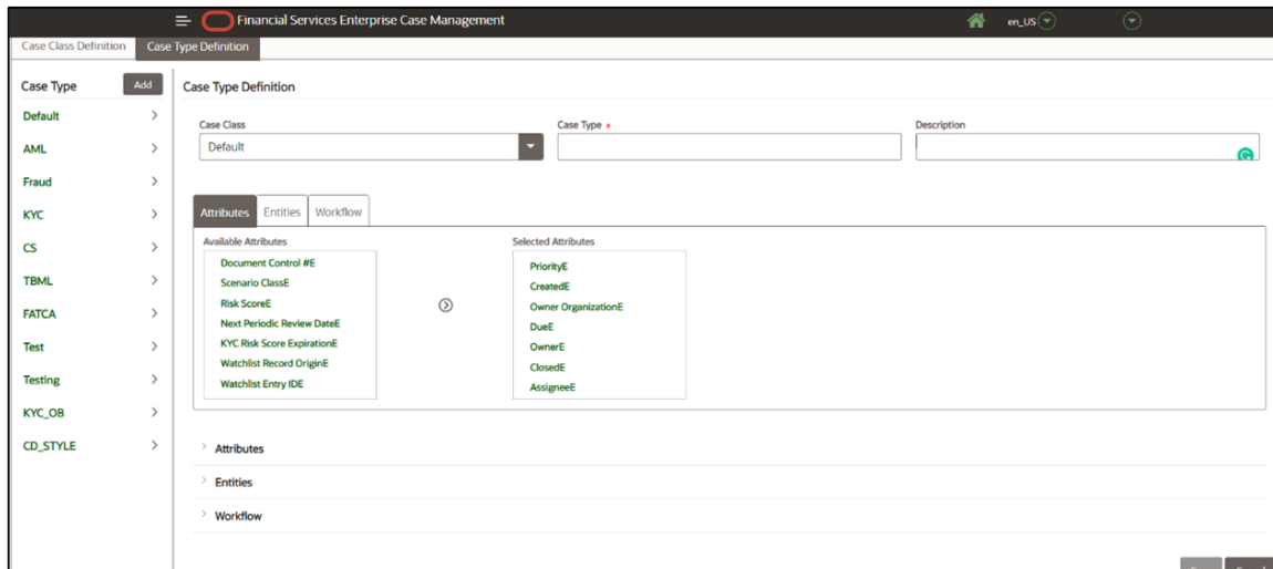
Figure 69: Attributes Page
