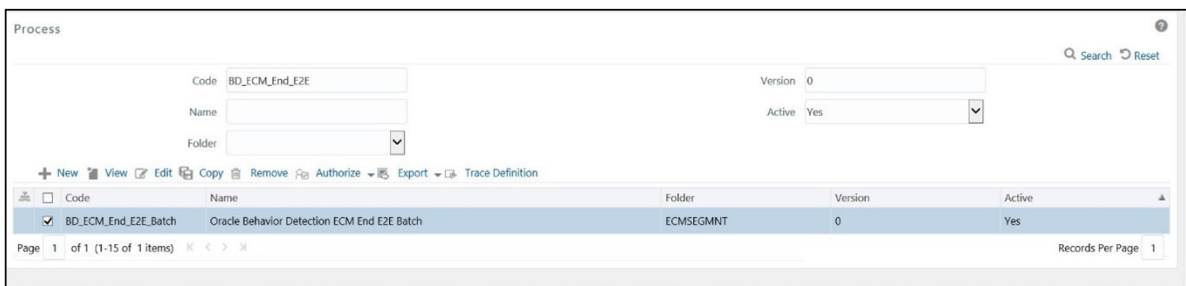
Figure 24: Process
