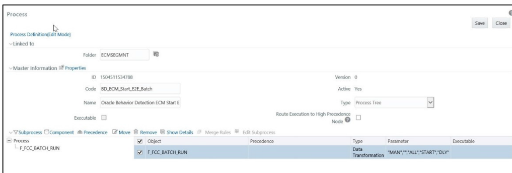
Figure 22: Process screen
