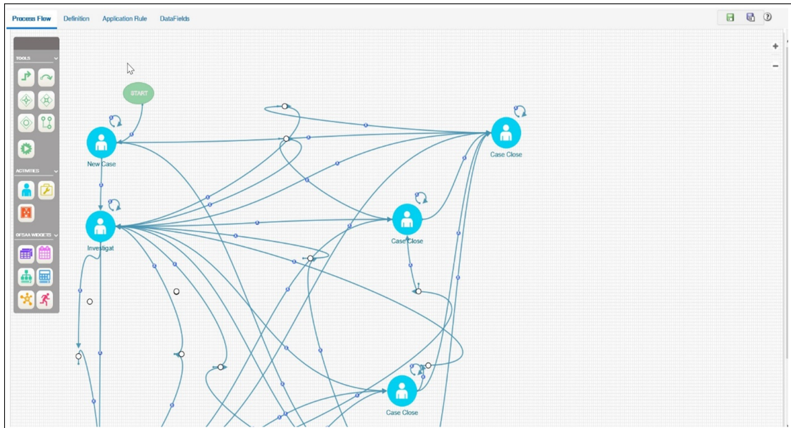
Figure 57: Editing Workflow
