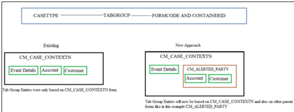
Figure 135: Workflow
