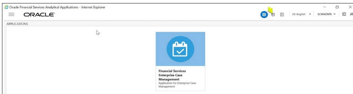
Figure 45: Applications
