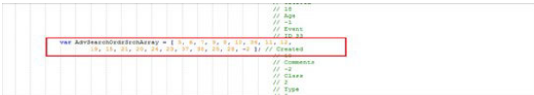
Figure 108: AdvSearchOrdSrchArray
