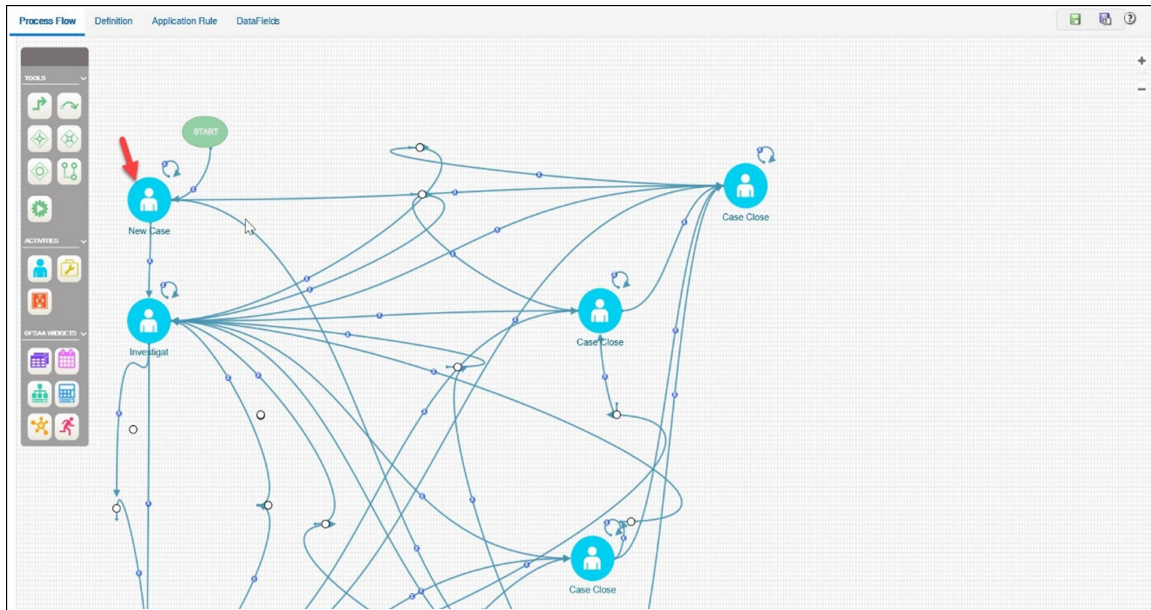
Figure 52: Adding Activity
