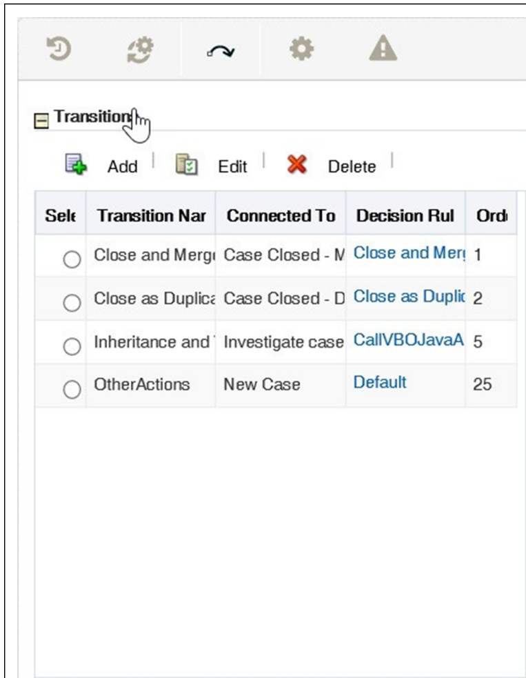
Figure 54: Add Transition
