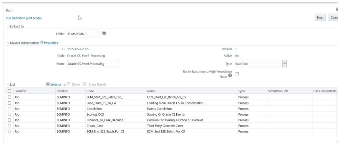
Figure 27: OCS Connector
