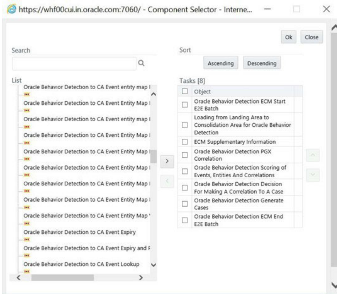
Figure 126: Component Selector
