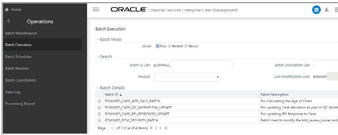
Figure 97: Batch Execution
