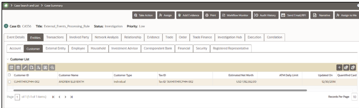
Figure 131: Customer Tab
