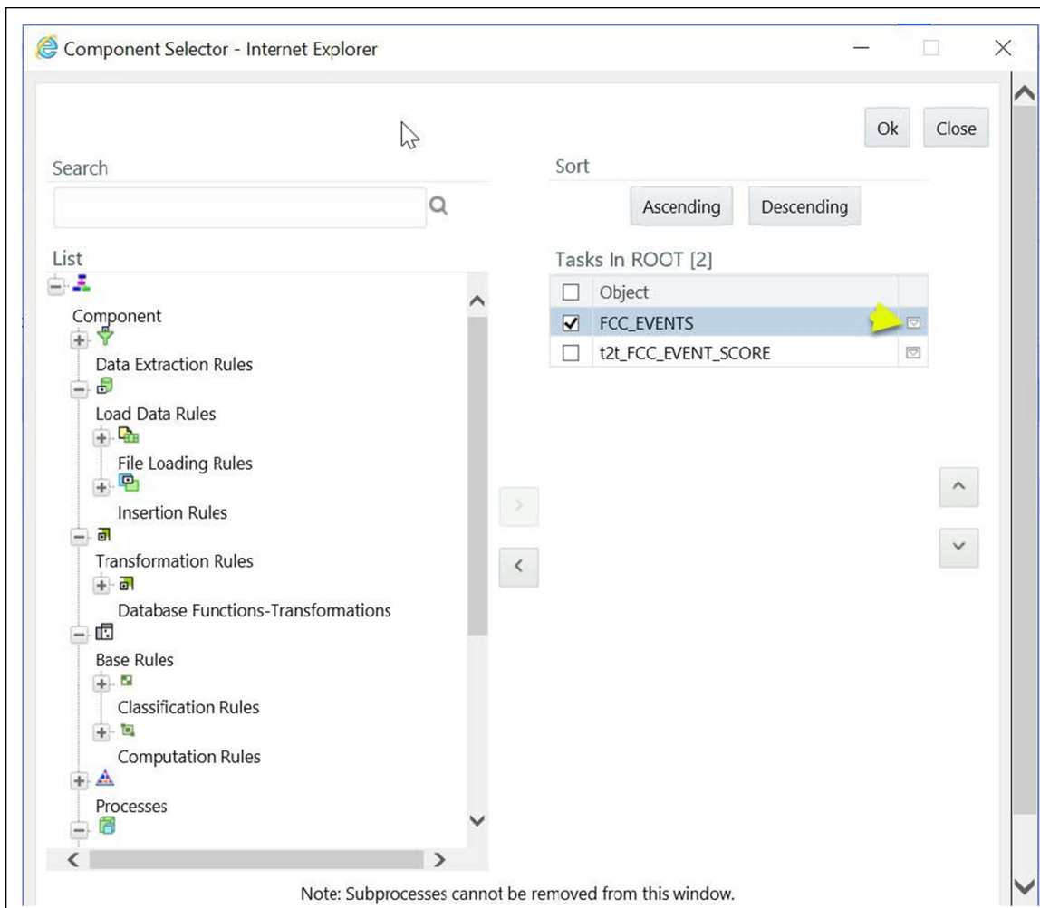
Figure 40: Components
