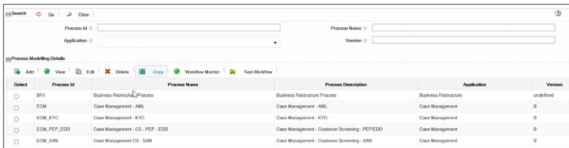
Figure 47: Process Modelling
