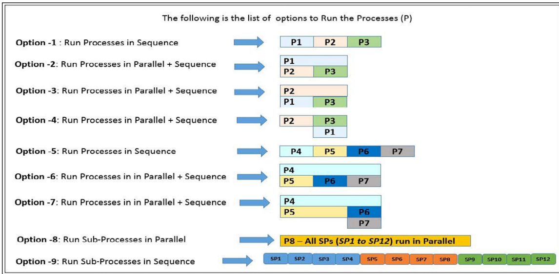
Figure 32: Options- processes
