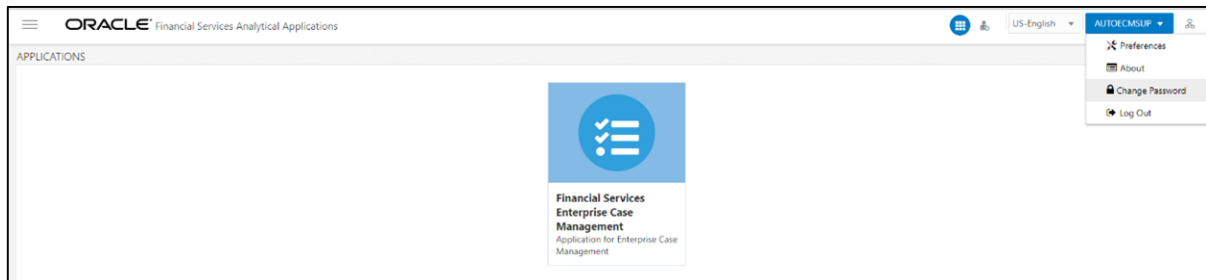
Figure 5: Applications page
