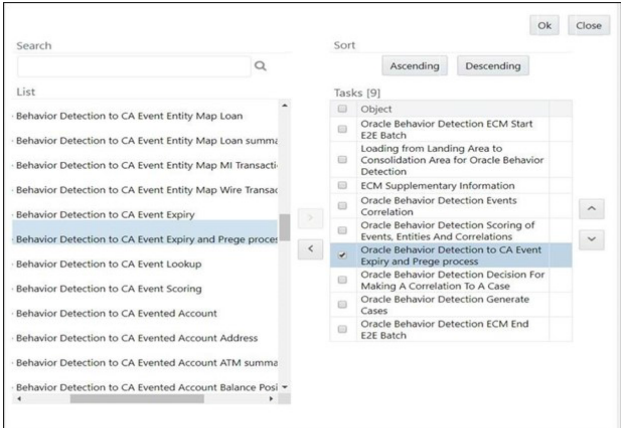
Figure 127: Components
