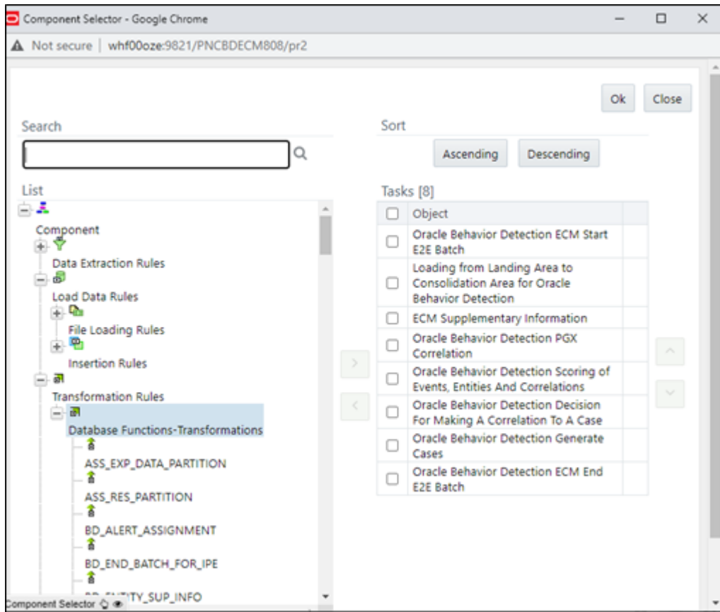
Figure 34: Component Selector
