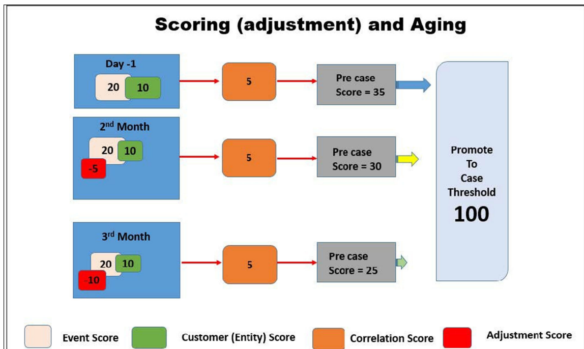
Figure 36: Adjustment Scoring
