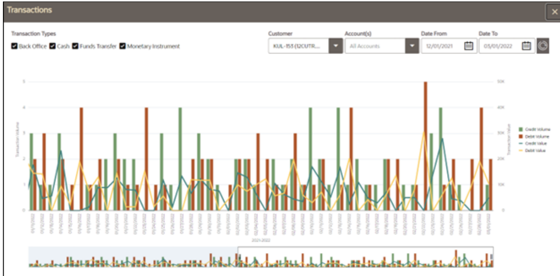
Figure 134: Transaction Chart
