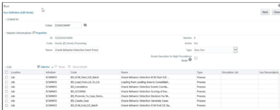
Figure 26: BD Processes
