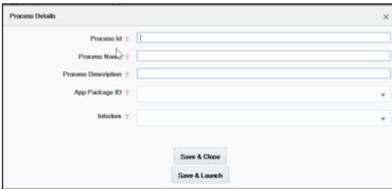
Figure 49: Process Details
