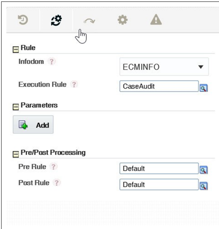
Figure 53: Implementing Activity
