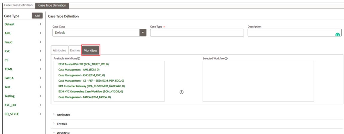
Figure 71: Workflow Page
