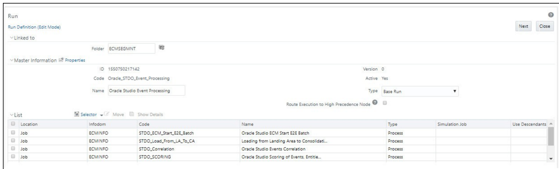
Figure 29: Studio Connector
