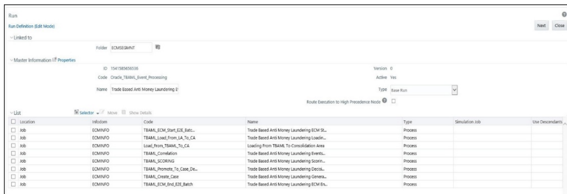
Figure 28: TBAML Connector
