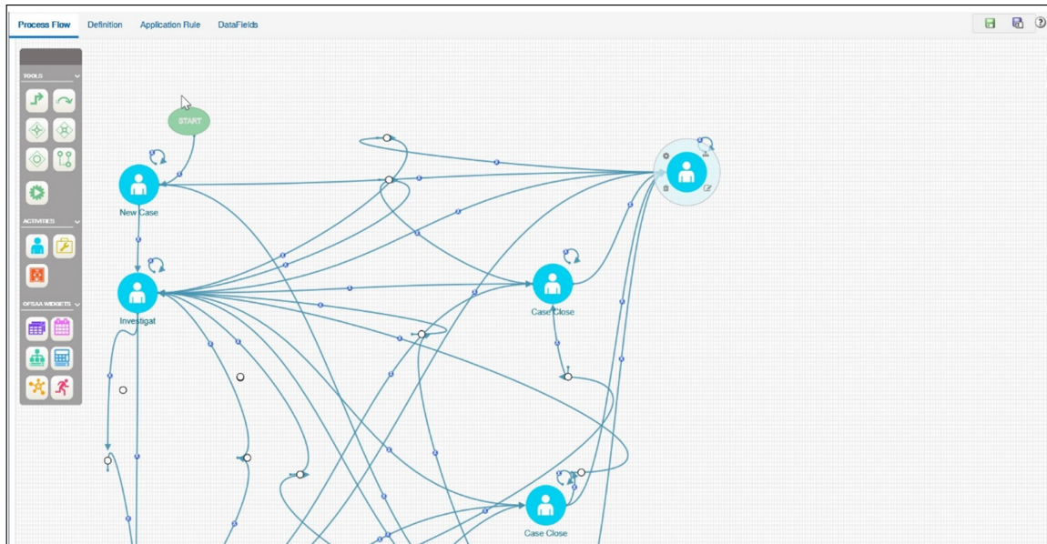
Figure 51: Starting Process
