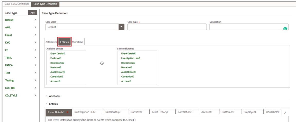
Figure 70: Entities Page
