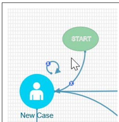
Figure 55: Adding Transition
