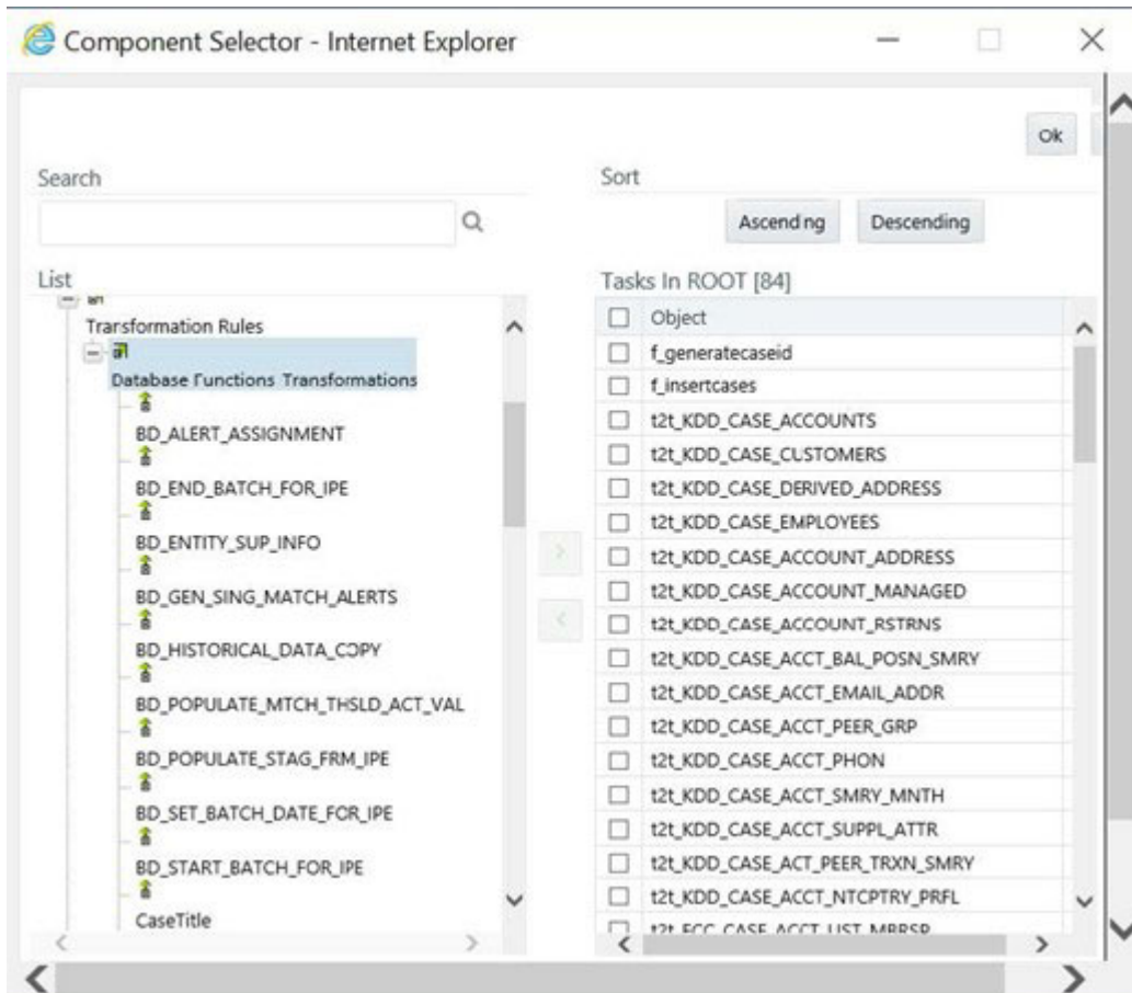
Figure 120: Component Selector
