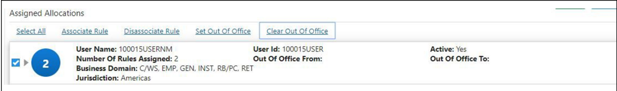
Figure 78: Assigned Allocations
