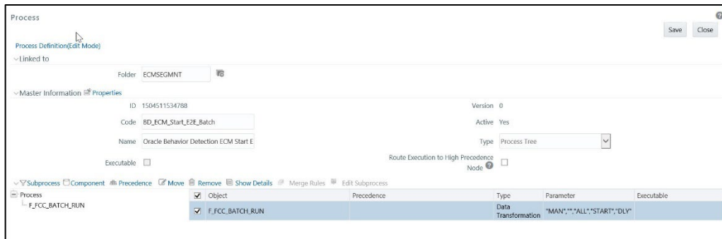
Figure 24: Process Screen
