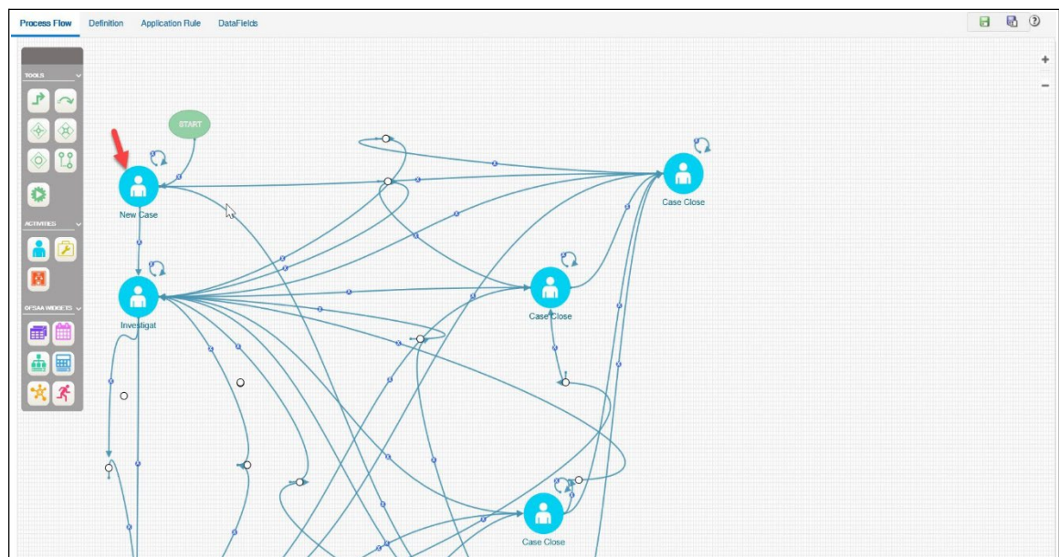
Figure 33: Adding Activity
