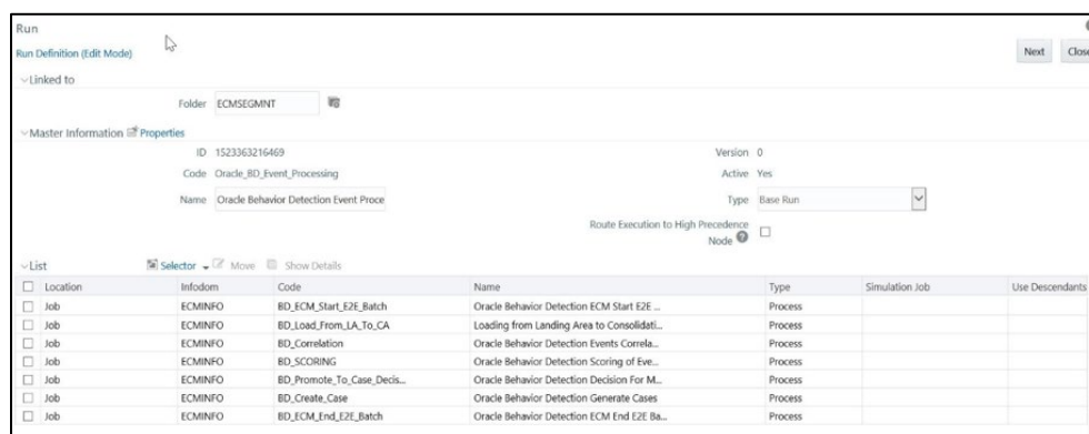
Figure 27: BD Processes
