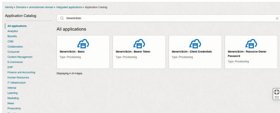
Figure 17: Select Application
