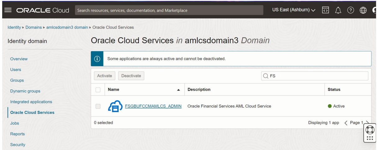
Figure 19: FSGBUFCCMAMLCS_ADMIN
