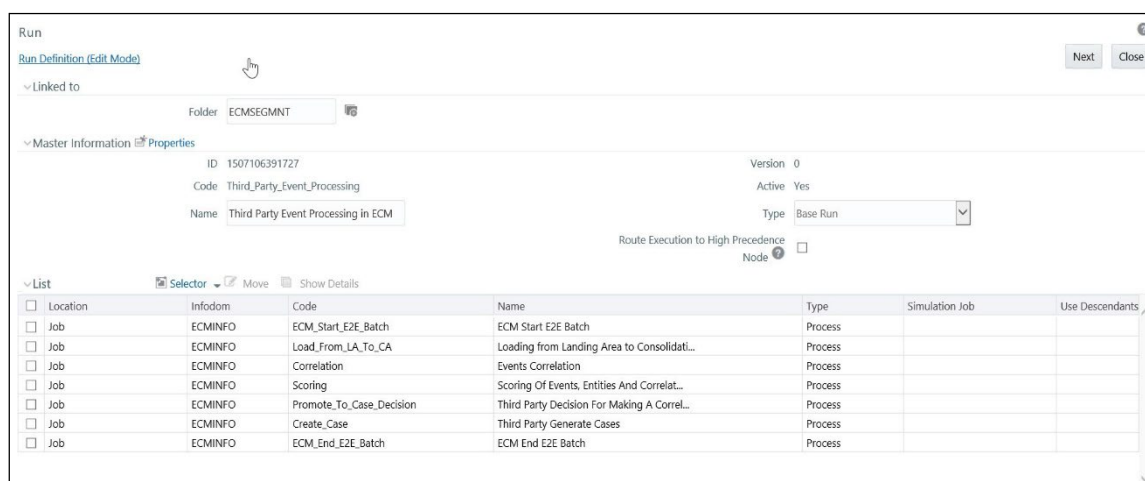
Figure 15: Third-party Connector
