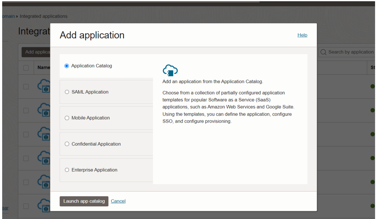
Figure 16: Add Application
