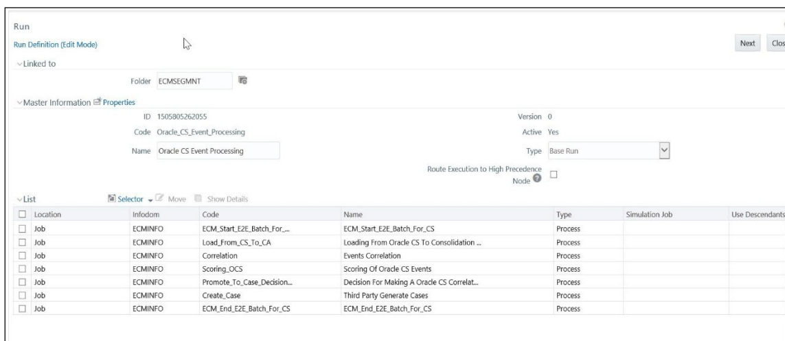
Figure 28: OCS Connector
