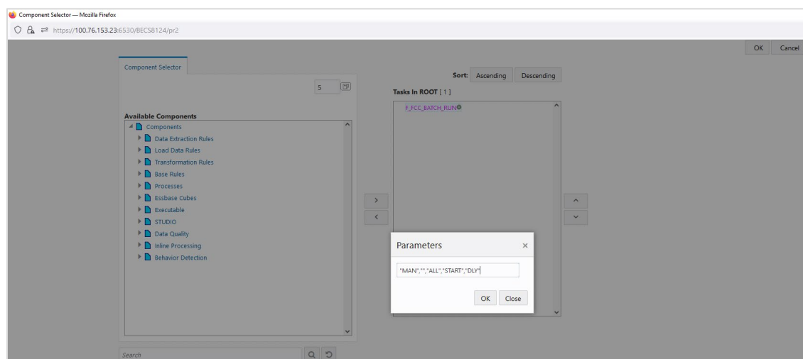
Figure 25: Parameters
