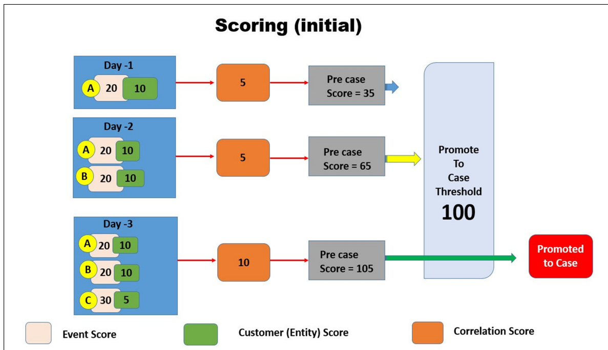
Figure 44: Initial Scoring Process
