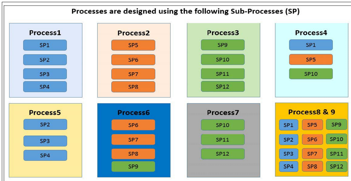
Figure 40: Oracle Behavior Detection Subprocesses
