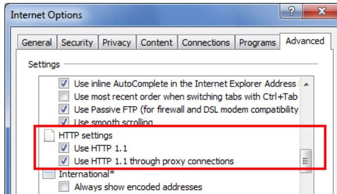
Figure 19 – HTTP 1.1 Settings
