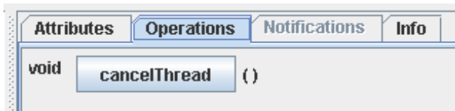
Figure 47 – Example cancelThread
