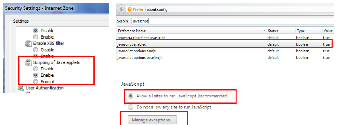
Figure 20 – Javascript Settings
