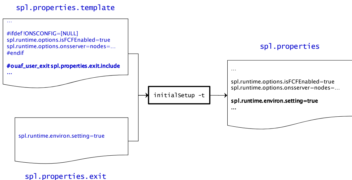
Figure 40 – Include files
