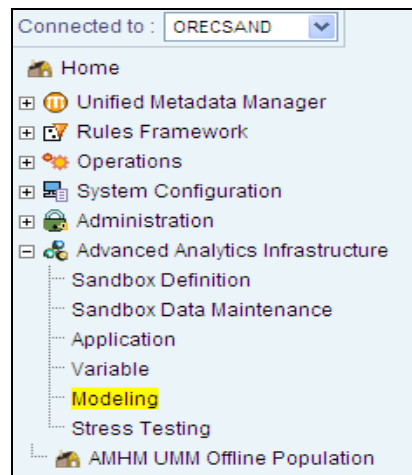
Figure 19: Sandbox Definition
