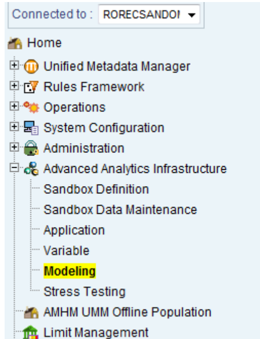
Figure 2: OREC modeling
