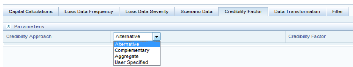
Figure 10: Credibility Factor
