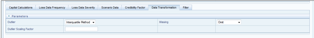
Figure 11: Data Transformation
