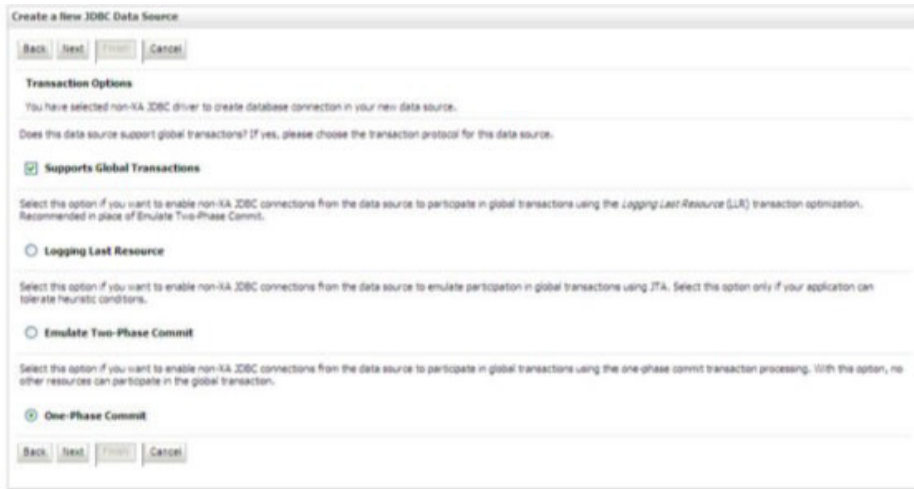
Figure B–12 Transaction Options
