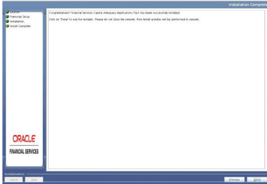
Figure 4–62 Installation Complete
