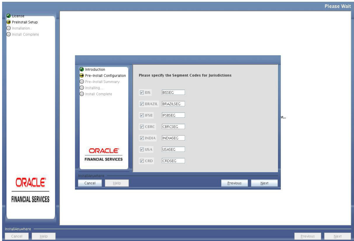
Figure 4–43 Jurisdictions Details
