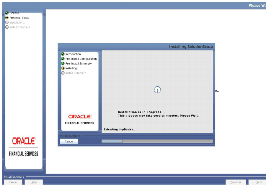
Figure 4–56 Installation Progress
