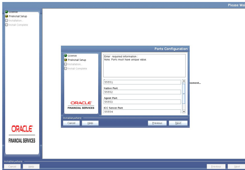
Figure 4–27 Ports Configuration
