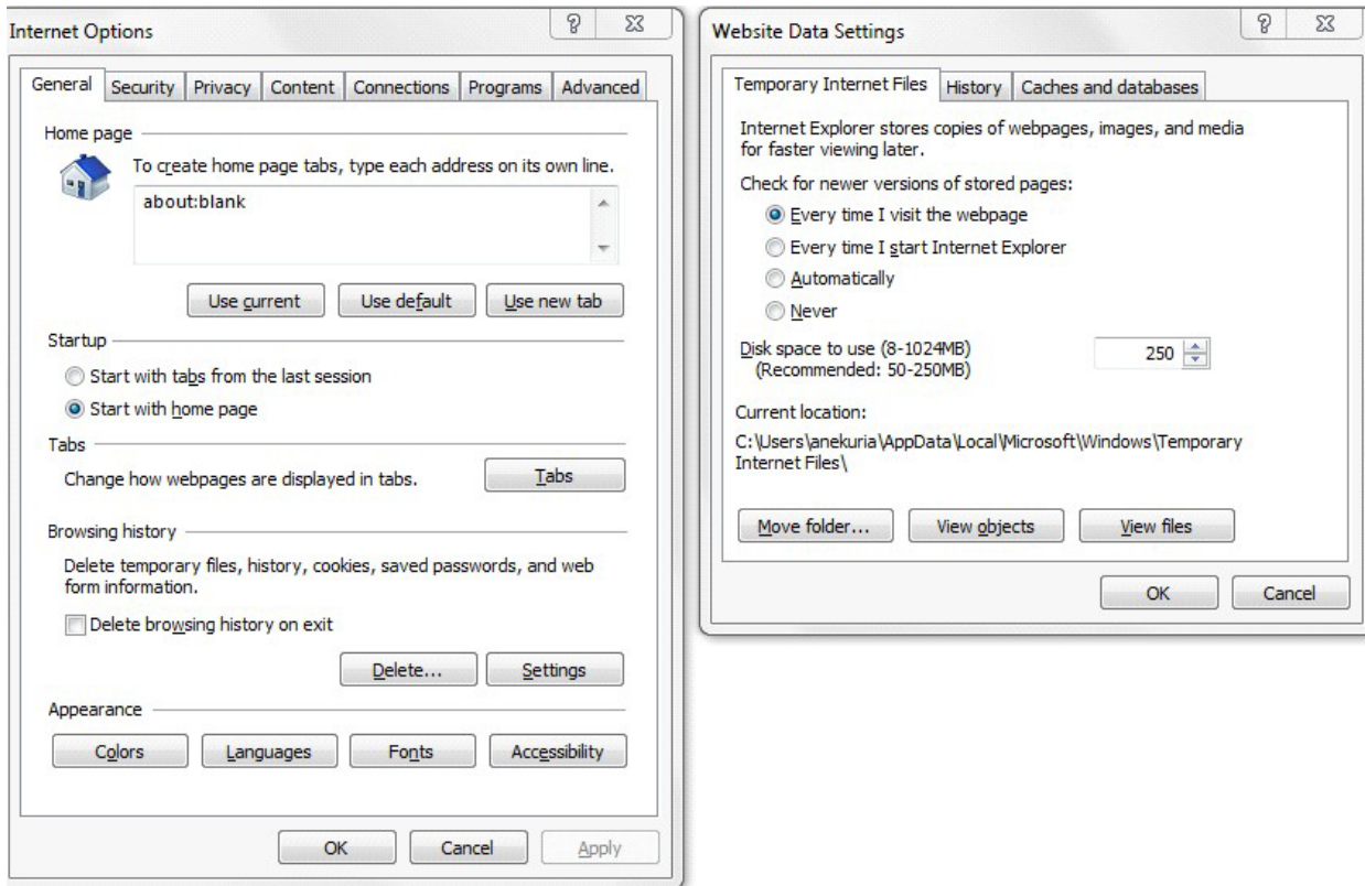
Figure I-1 Internet Options
