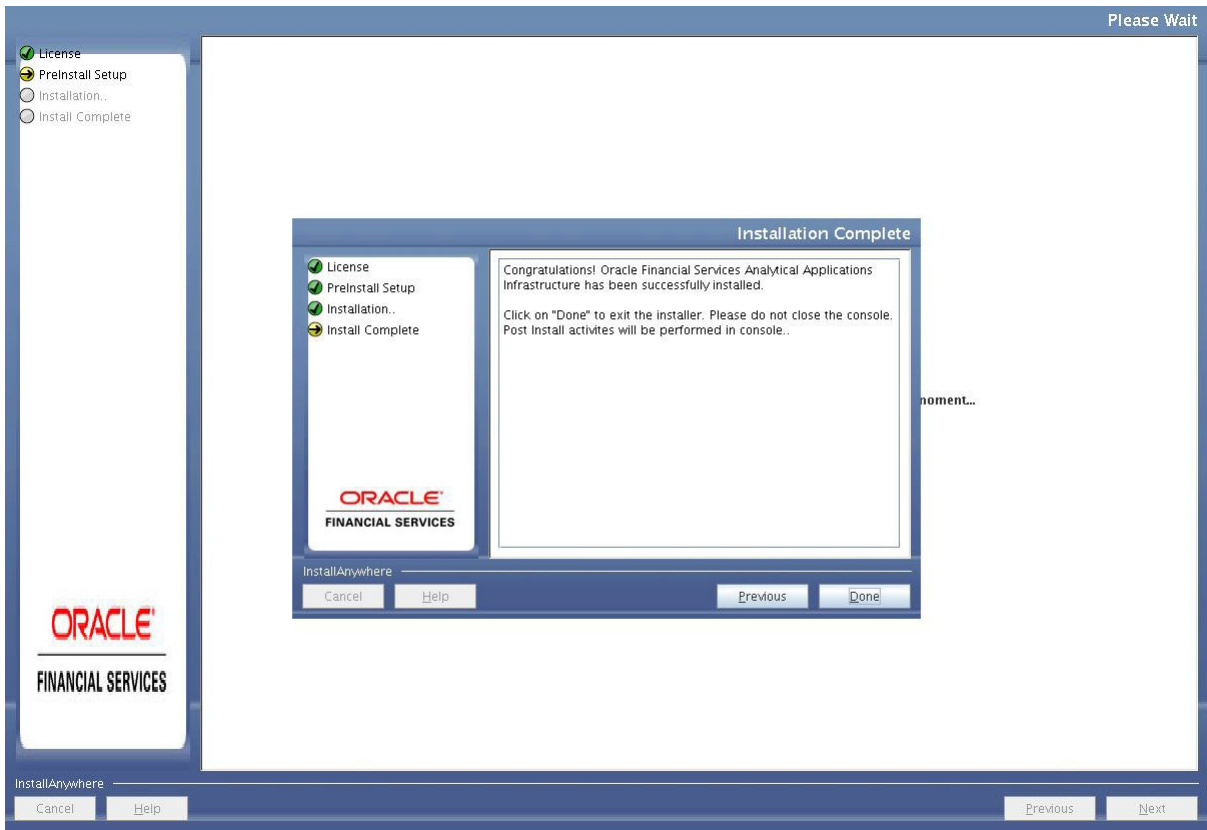
Figure 4–34 Installation Complete
