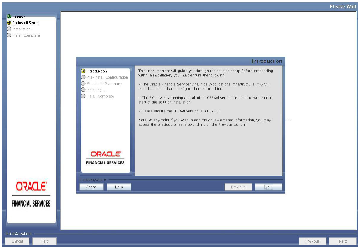
Figure 4–37 Installation Introduction
