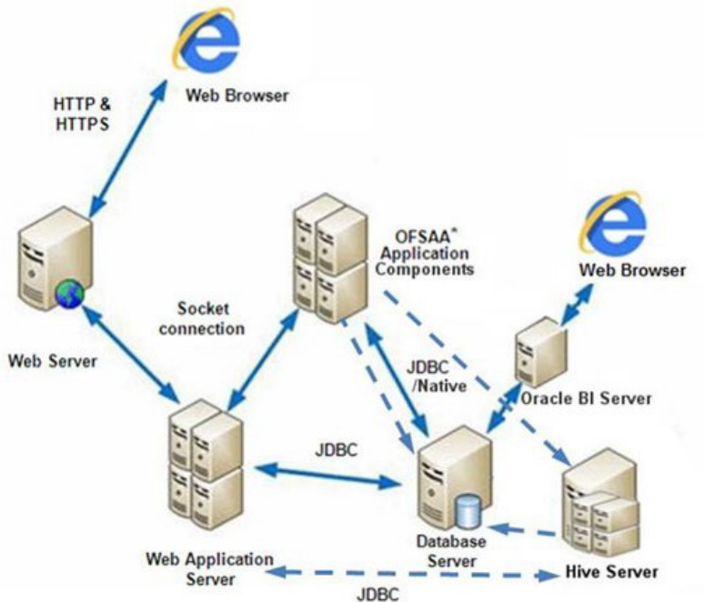
Figure 2-2 Deployment Topology
