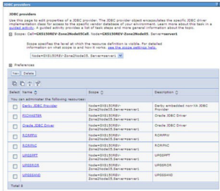
Figure 6–3 JDBC Providers
