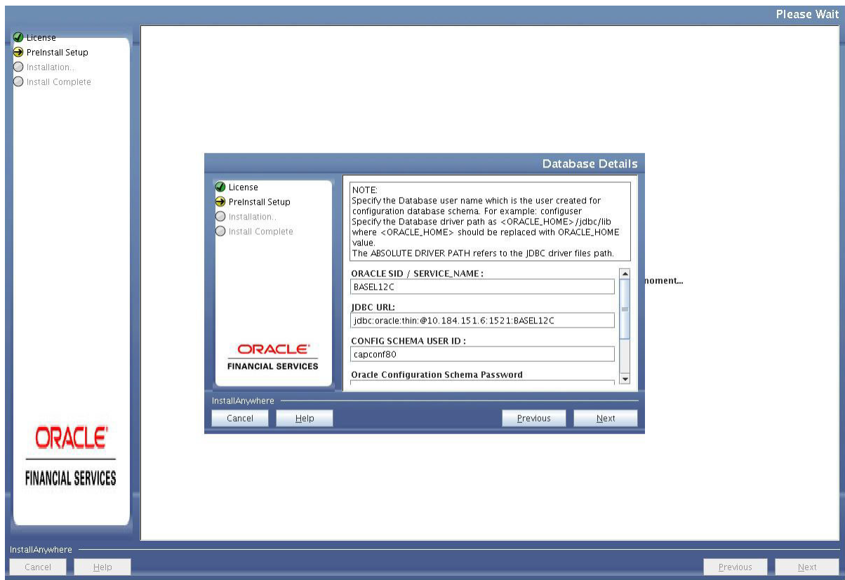
Figure 4–26 Database Details
